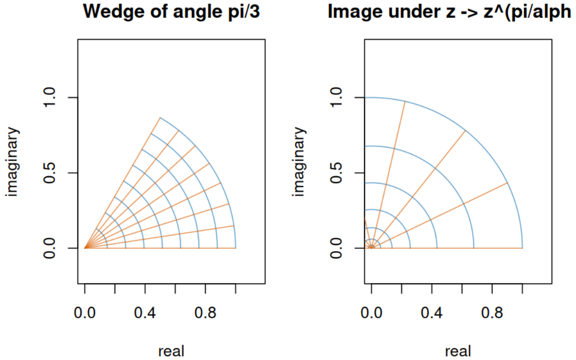
Figure 10: A wedge grid straightened by a power map
