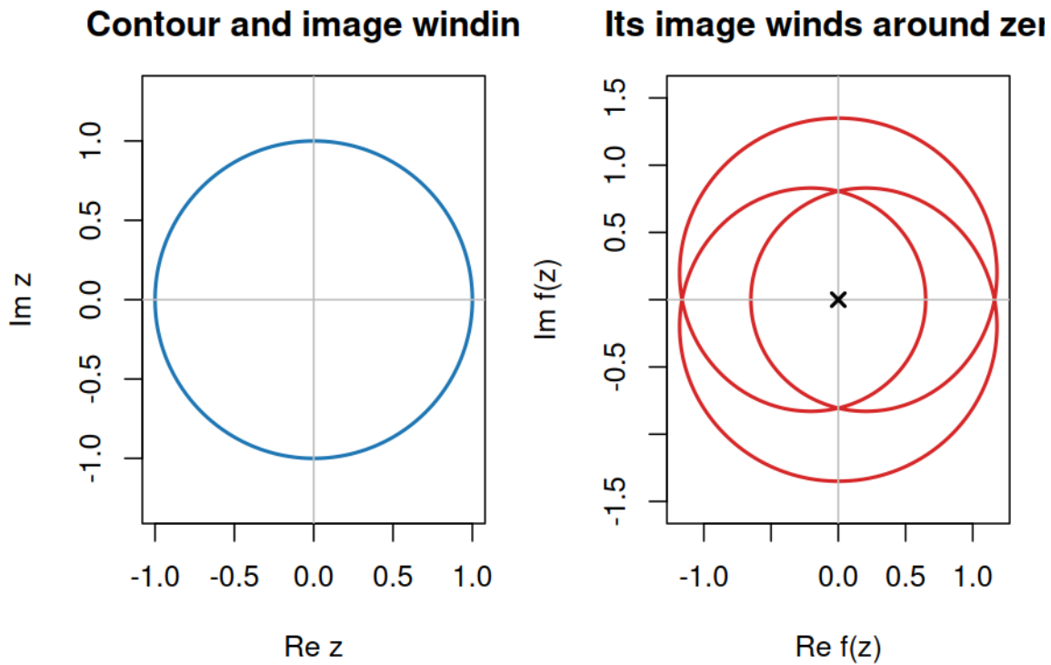
Figure 8: A contour and the image curve used by the argument principle
