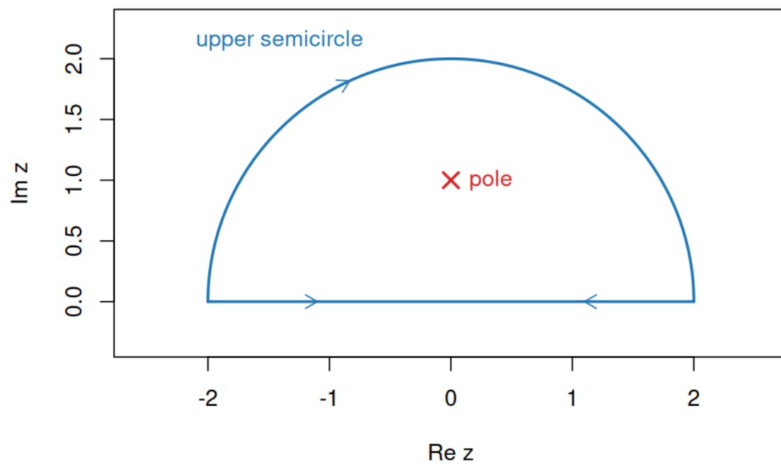
Figure 13: A semicircle contour selected by exponential decay
