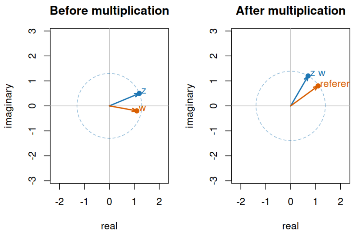
Figure 2: Multiplication by a complex number as rotation and scaling
