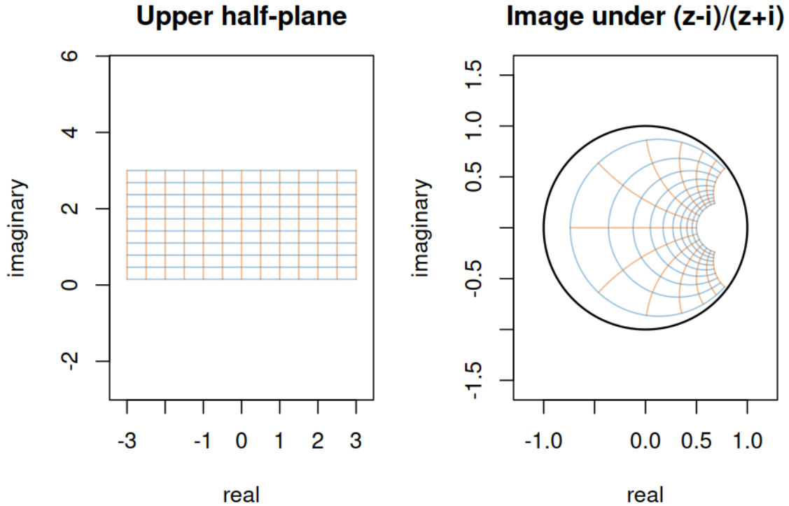
Figure 9: A grid in the upper half-plane and its image in the unit disk
