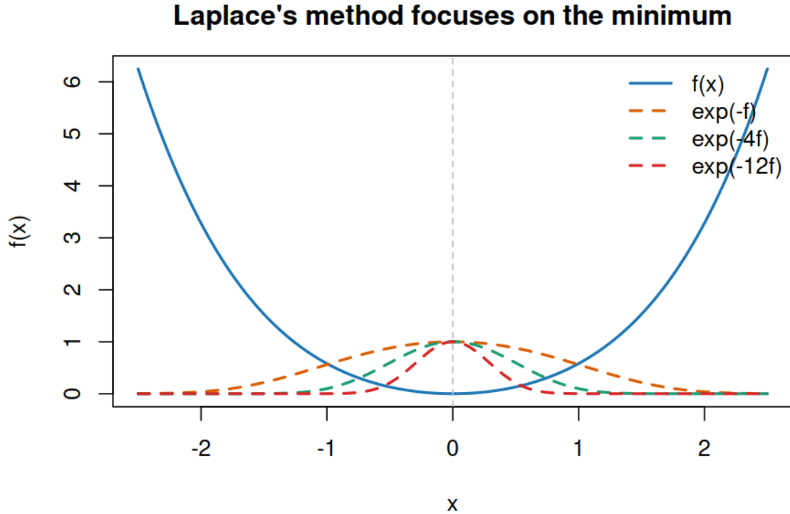
Figure 14: Laplace concentration near a non-degenerate minimum
