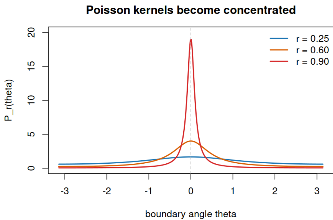
Figure 12: Poisson kernels concentrating near their boundary point
