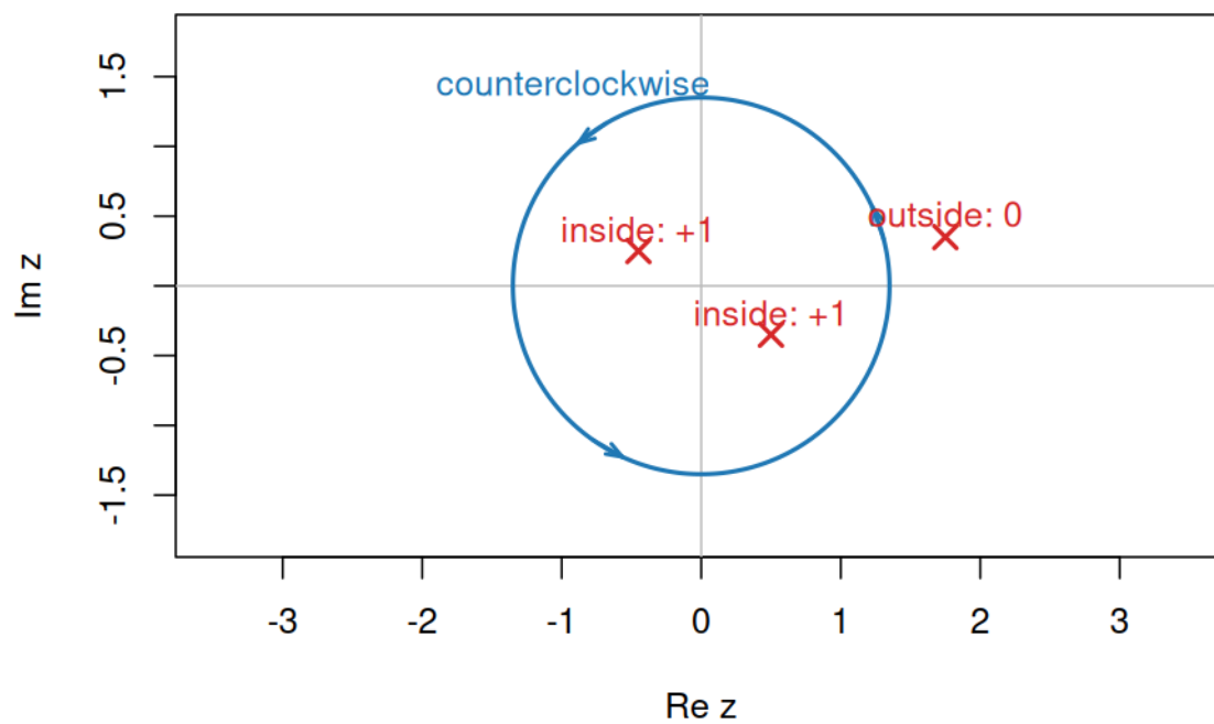
Figure 4: A directed contour with points of different winding number
