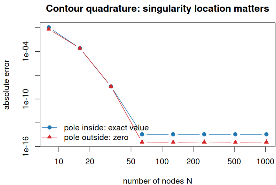
Figure 15: Periodic contour quadrature converges differently when the pole is inside or outside
