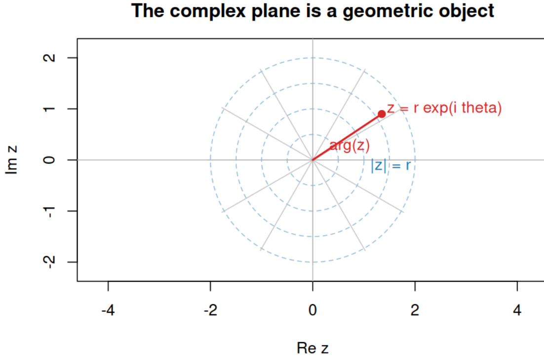
Figure 1: The complex plane with polar coordinates, concentric modulus circles, and argument rays
