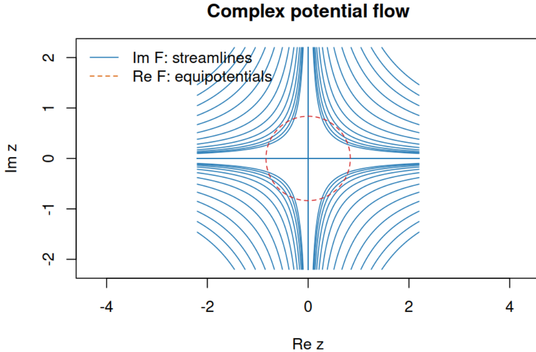
Figure 11: Streamlines and equipotentials for a complex potential
