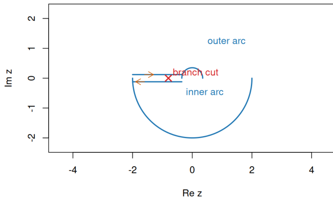
Figure 7: A keyhole contour following both banks of a branch cut
