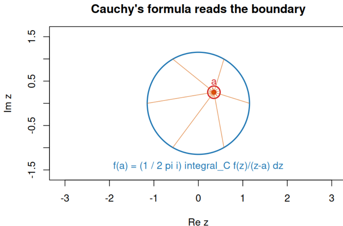
Figure 5: Cauchy's formula connects boundary values to an interior point
