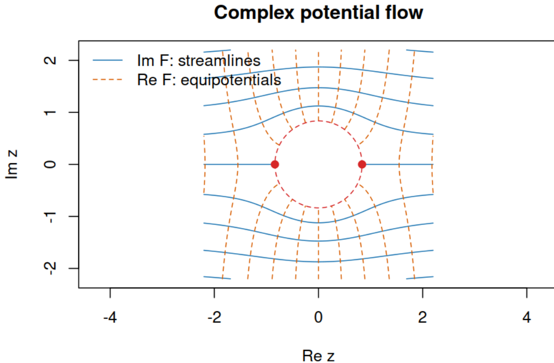
Figure 12: Streamlines and equipotentials for a complex potential
