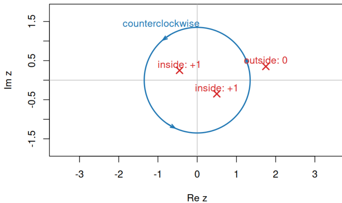
Figure 5: A directed contour with points of different winding number
