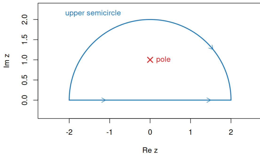
Figure 14: A semicircle contour selected by exponential decay
