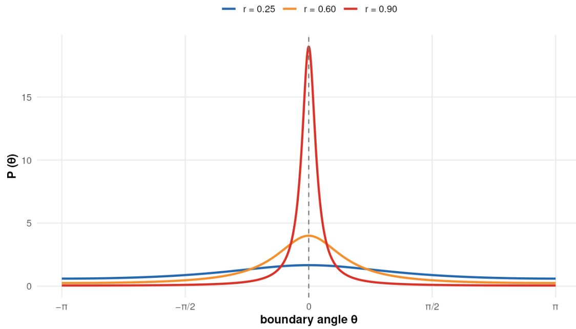
Figure 13: Poisson kernels concentrating near their boundary point
