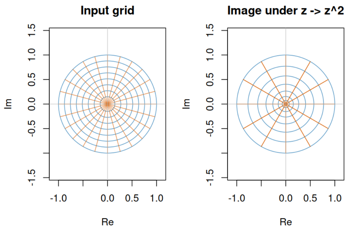
Figure 4: A square map takes a circular and radial grid to another conformal grid
