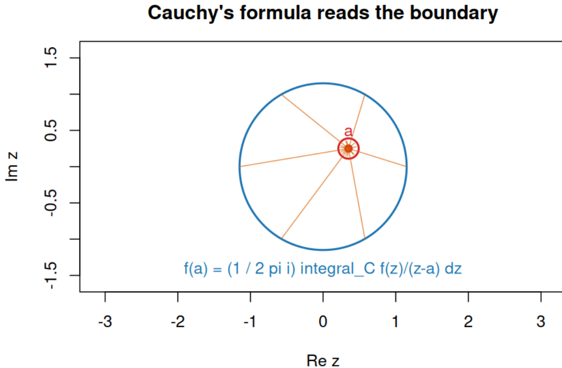
Figure 6: Cauchy's formula connects boundary values to an interior point
