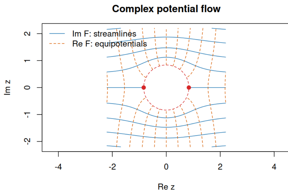
Figure 12: Streamlines and equipotentials for a complex potential
