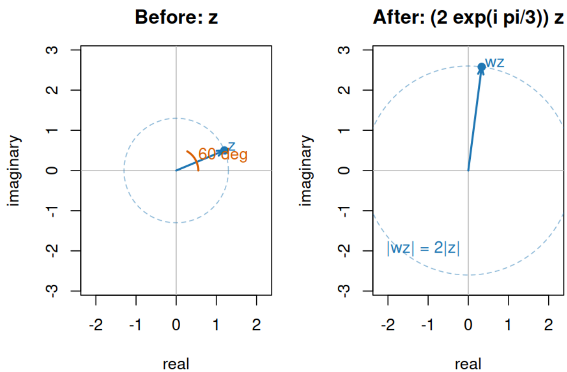
Figure 3: Multiplication by a complex number as rotation and scaling
