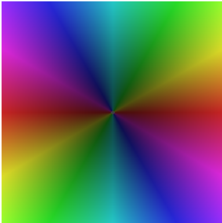
Figure 1: Domain colouring for the square map
