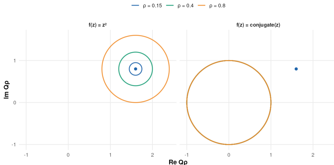
Figure: The difference quotient for z^2 approaches the single complex number 2z_0 as the step radius shrinks. For \bar{z} , the quotient remains direction-dependent, tracing the unit circle instead of converging to one value.
