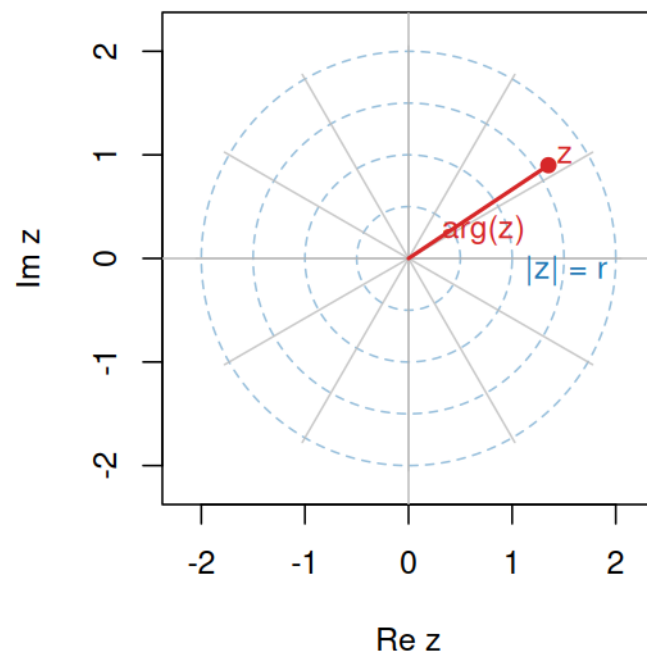
Figure 2: The complex plane with polar coordinates, concentric modulus circles, and argument rays
