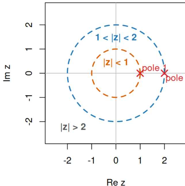
Figure 7: Three Laurent annuli separated by singularity circles
