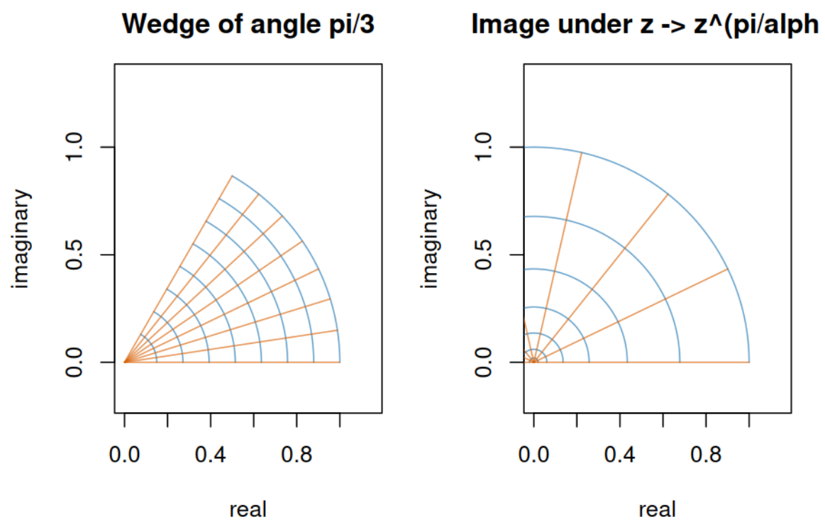
Figure 11: A wedge grid straightened by a power map
