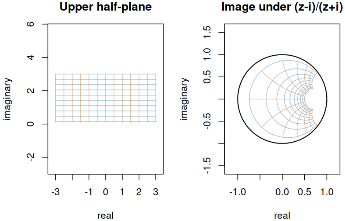
Figure 10: A grid in the upper half-plane and its image in the unit disk
