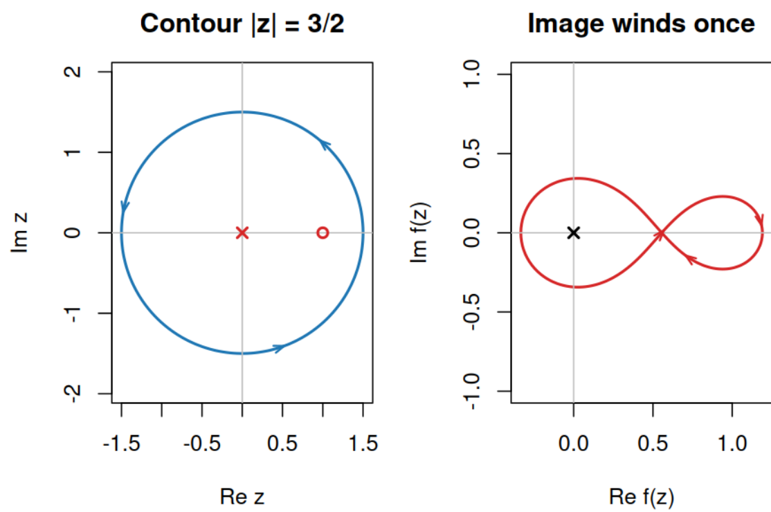
Figure 9: A contour and the image curve used by the argument principle
