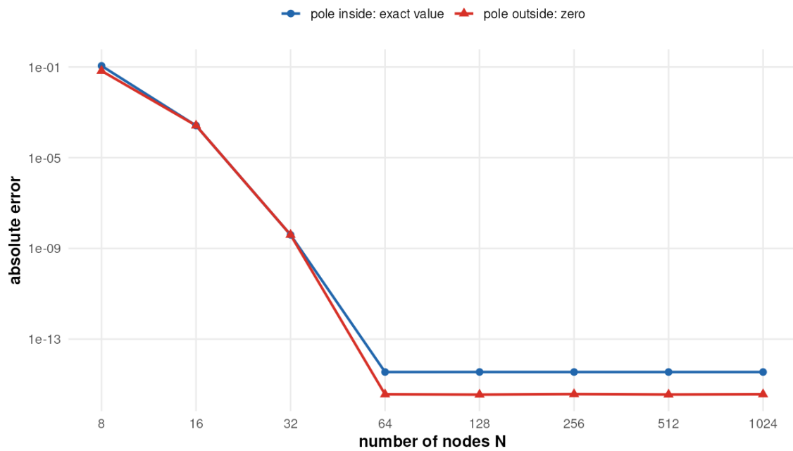
Figure 16: Periodic contour quadrature converges differently when the pole is inside or outside
