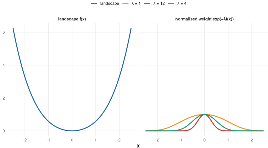
Figure 15: Laplace concentration near a non-degenerate minimum
