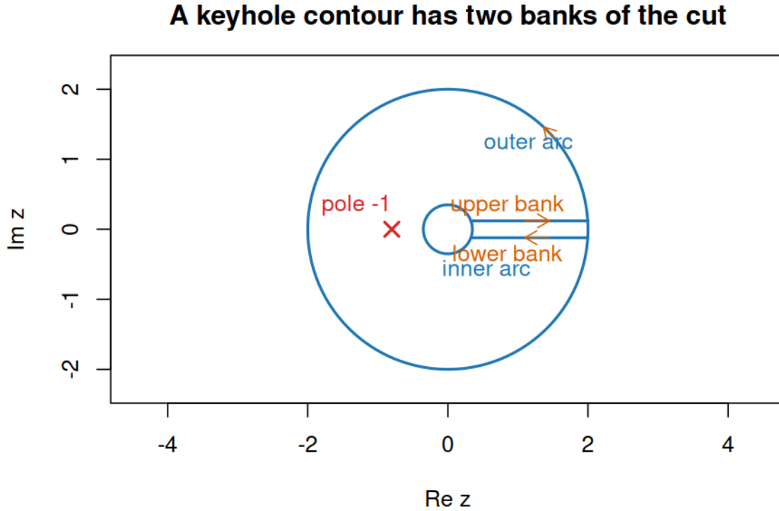
Figure 8: A keyhole contour following both banks of a branch cut
