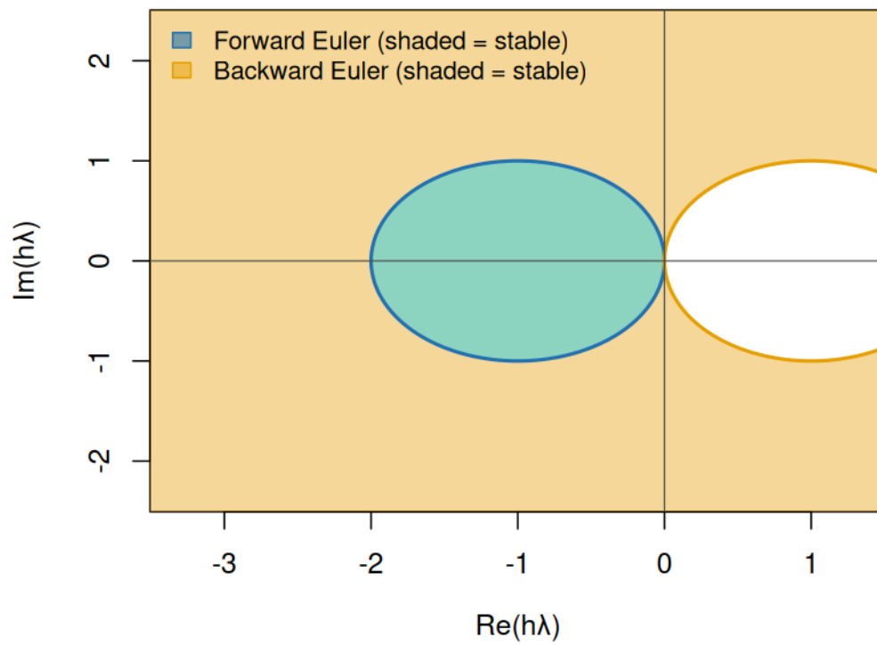
Figure 4: Stability regions: forward Euler vs backward Euler in the complex plane
