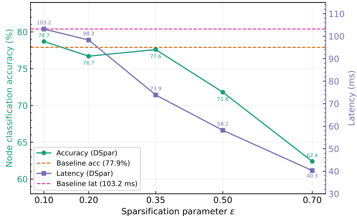
Effect of DSpar sparsification (Cora)
