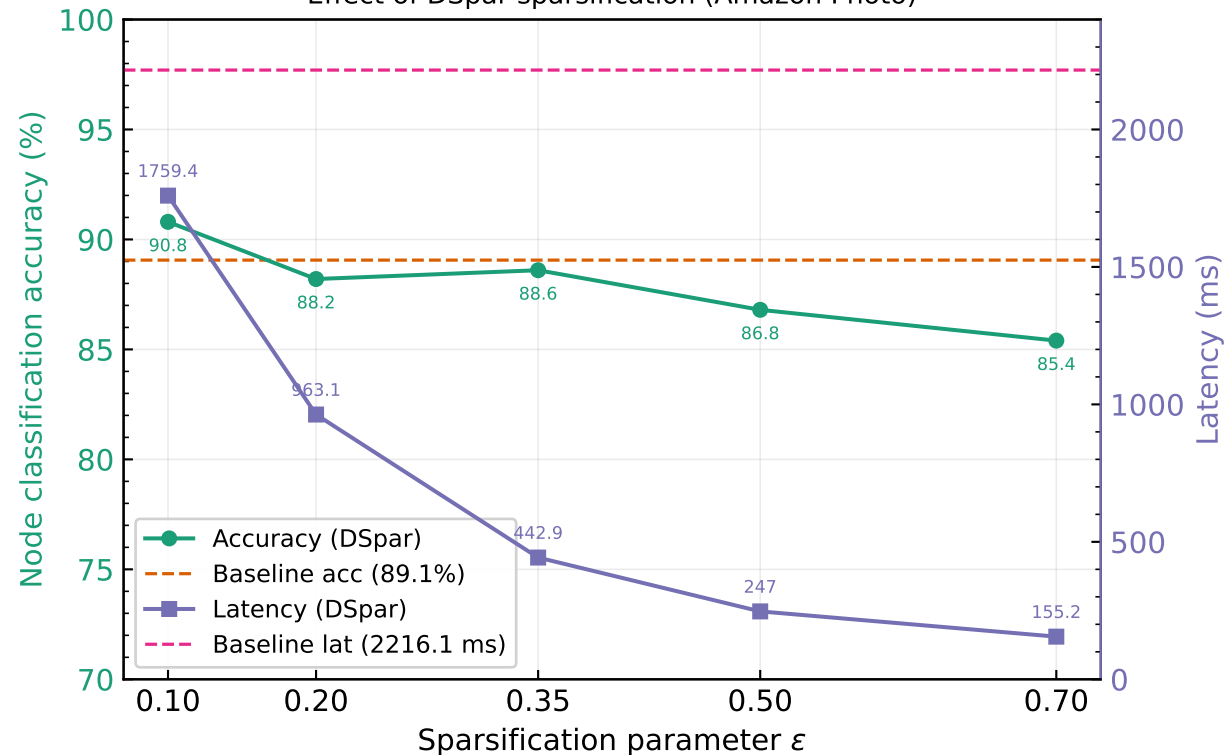
Effect of DSpar sparsification (Amazon Photo)
