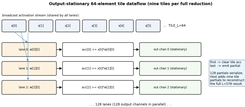
Figure 3. Tiled output-stationary dataflow: 64-element chiplet partials, nine-way host accumulation
