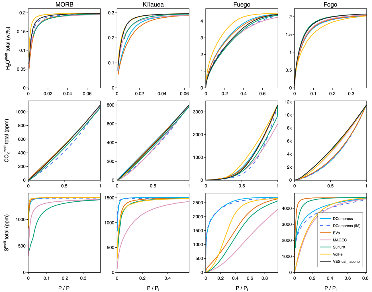
Figure 3: H 2 O total, CO 2 total, and S total concentrations in the melt as a function of normalized pressure during degassing runs with all tools. Modeled dissolved melt H 2 O and CO 2 are also shown for runs using the VESlcal implementation of the Iacono-Marziano model, which only considers H and C (black line). Note that x-axis maximum values are cropped to the point of the onset of significant degassing and differ between plots.
