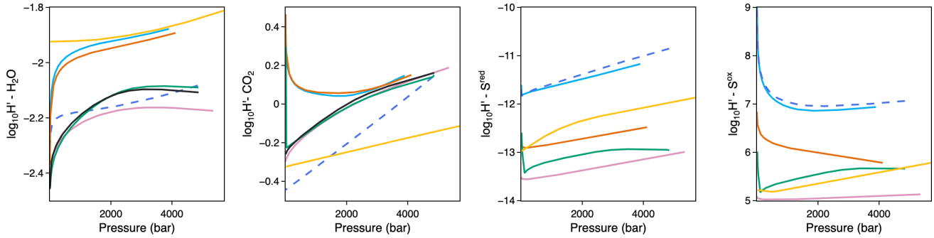
Figure 7: Volatile proportionality factors (eq. 15) with all tools for Fuego basalt showing the change in \text{H}_2\text{O} , \text{CO}_2 , reduced S ( S^{\text{red}} ), and oxidized S ( S^{\text{ox}} ) proportionality factors ( H'_i ) as a function of pressure during degassing.
