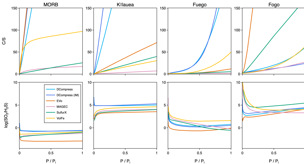
Figure 5: Calculated values of C/S and \log(SO_2/H_2S) molar ratios in the vapor phase as a function of normalized pressure of degassing for each volcanic system.
