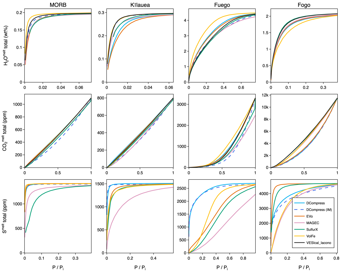
Figure 3: \text{H}_2\text{O} total, \text{CO}_2 total, and \text{S} total concentrations in the melt as a function of normalized pressure during degassing runs with all tools. Modeled dissolved melt \text{H}_2\text{O} and \text{CO}_2 are also shown for runs using the VESlcal implementation of the Iacono-Marziano model, which only considers H and C (black line). Note that x-axis maximum values are cropped to the point of the onset of significant degassing and differ between plots.
