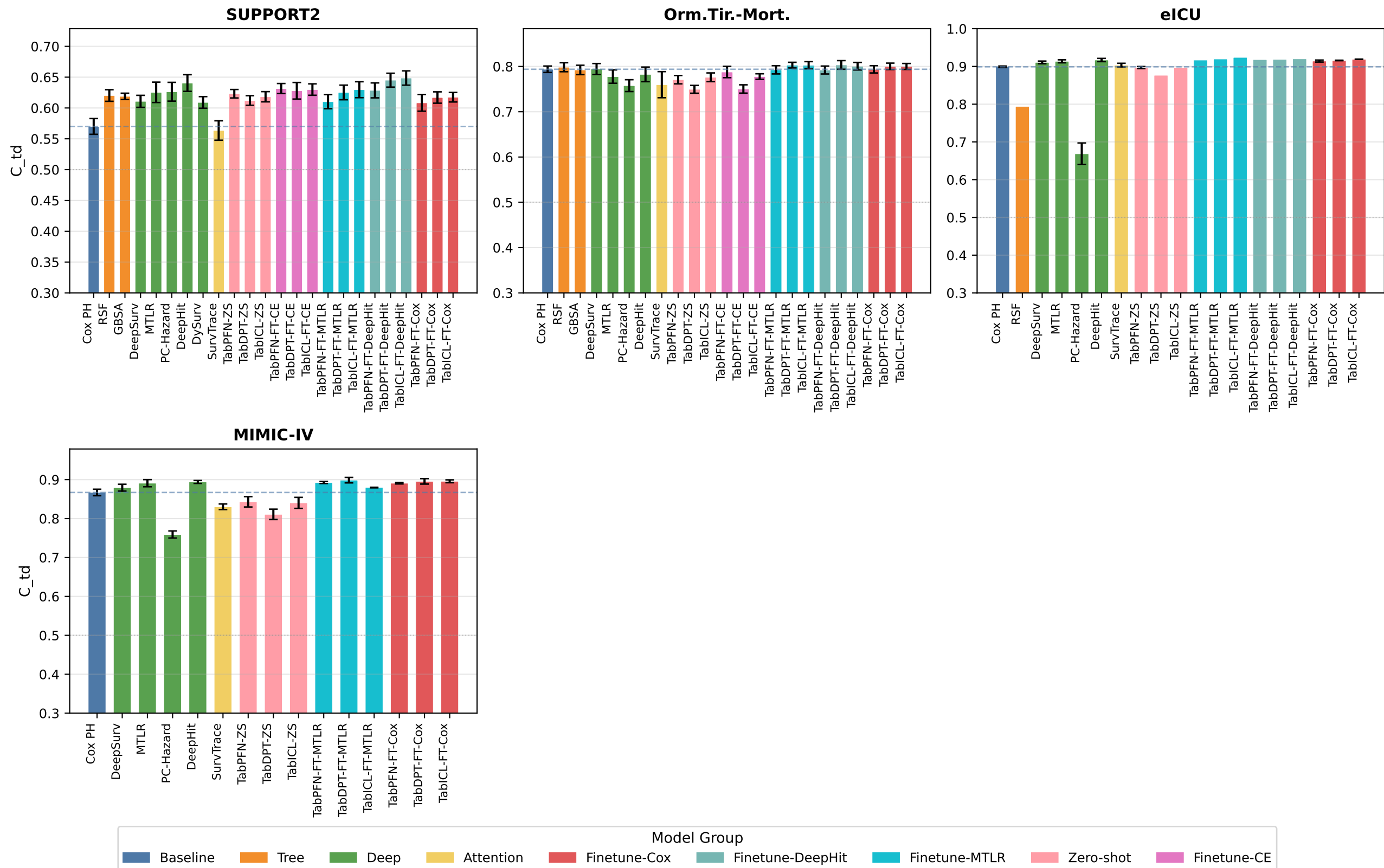
C_td Comparison (mean \pm std, 5-fold CV)
