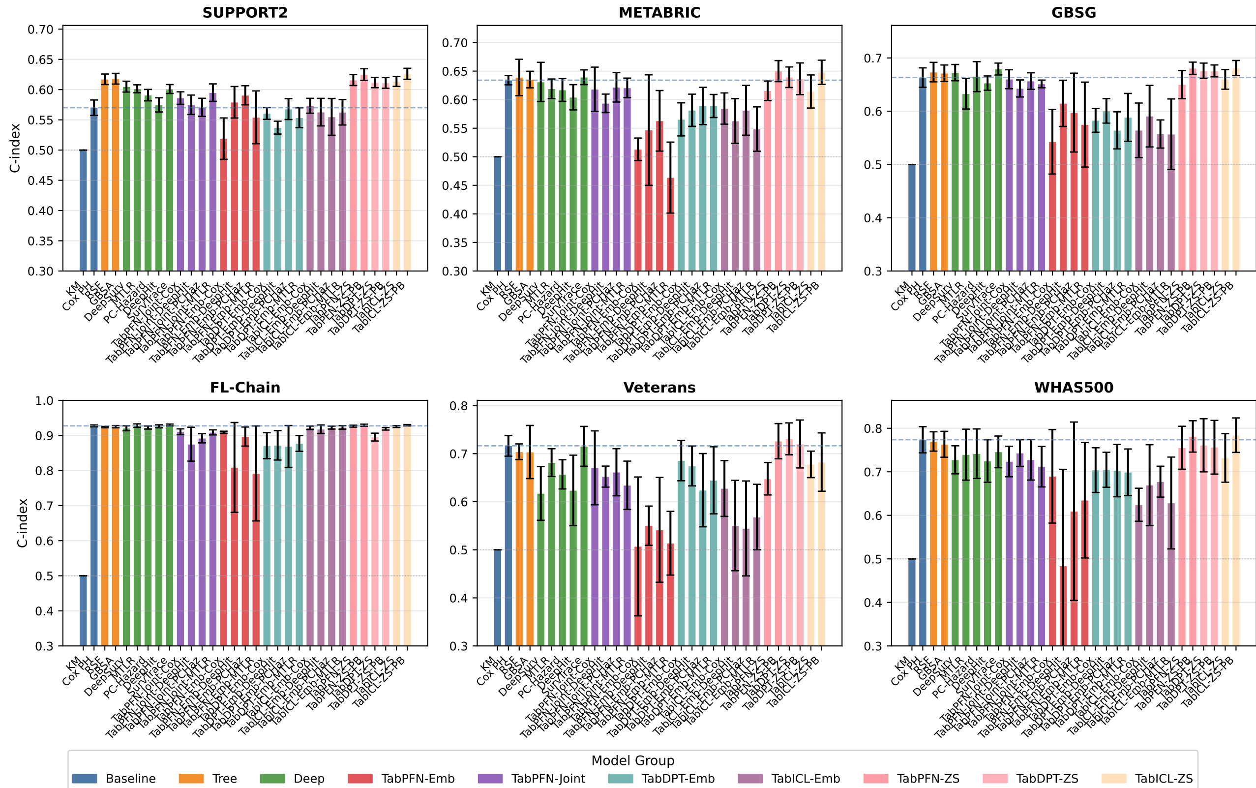
C-index Comparison (mean \pm std, 5-fold CV)
