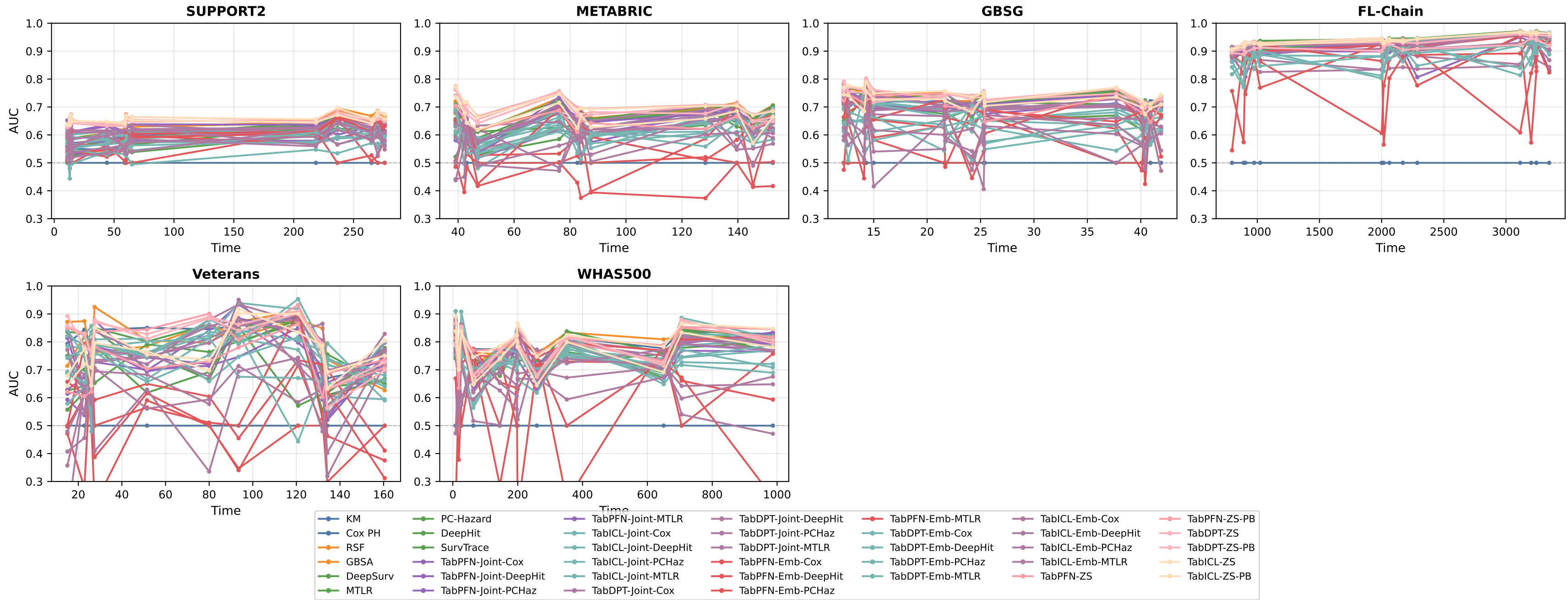
Time-dependent AUROC (mean across 5 folds)
