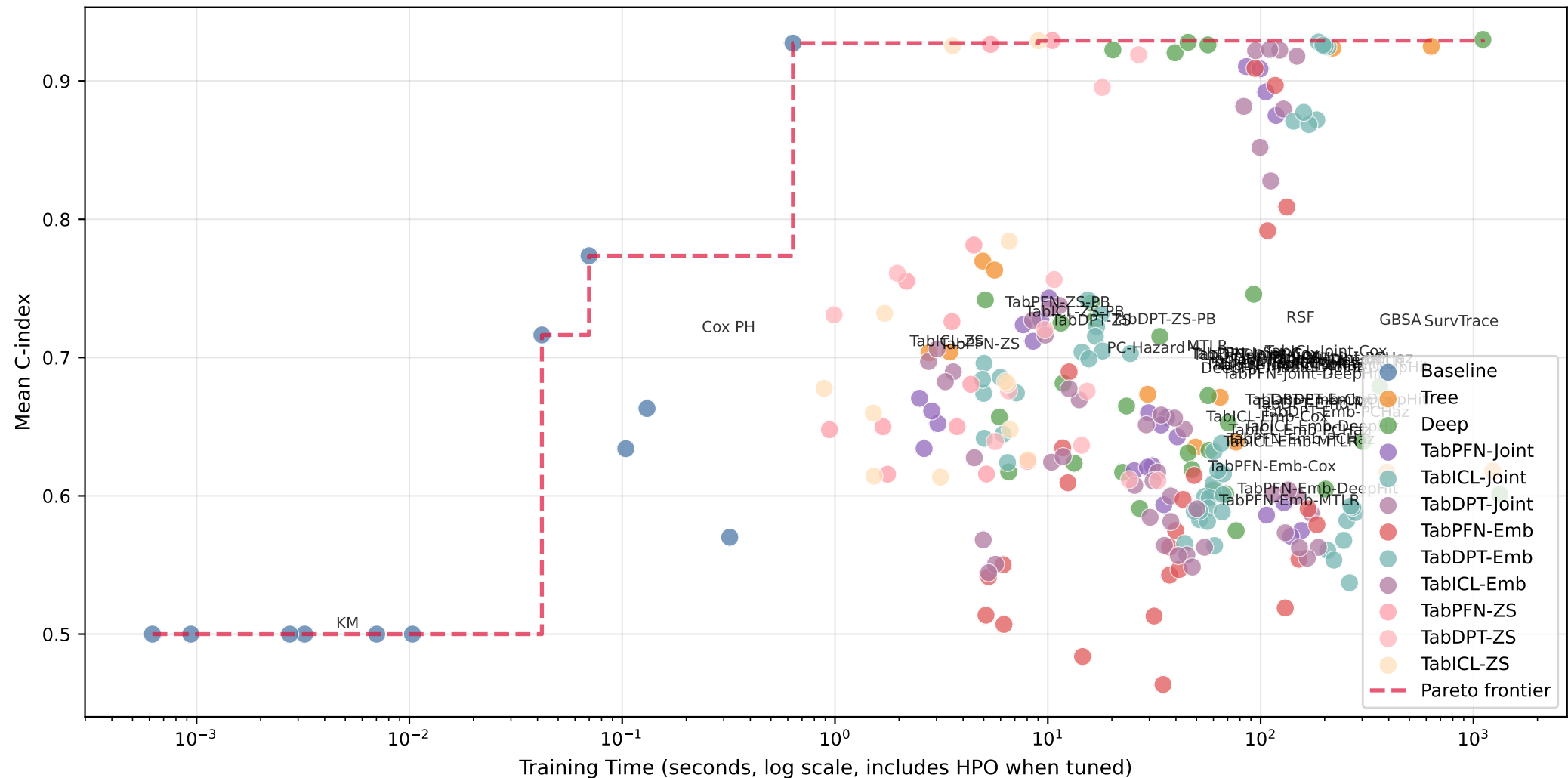
Performance-Efficiency Frontier (each point = model × dataset mean)
