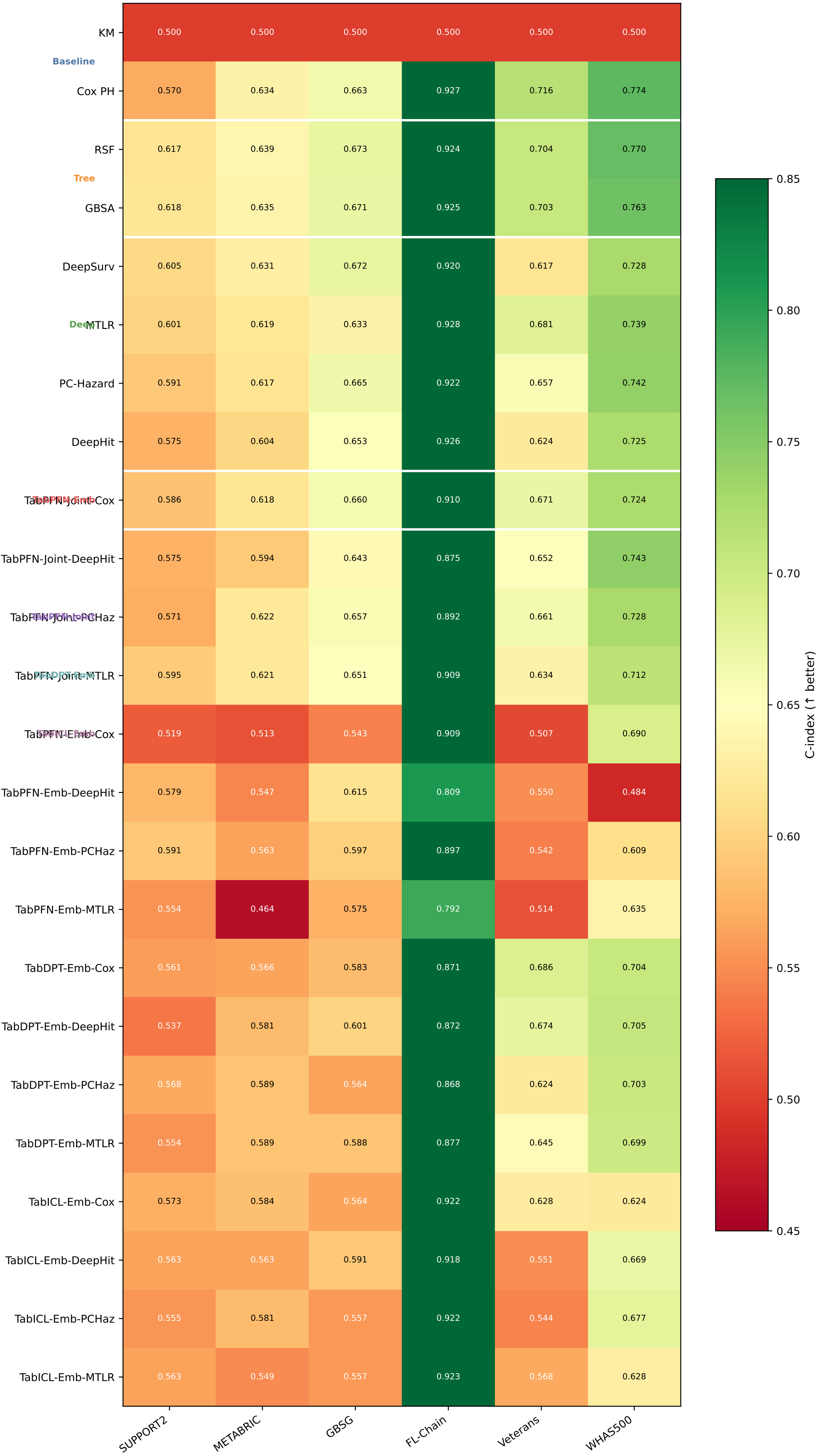
Mean C-index Across 5-fold CV
