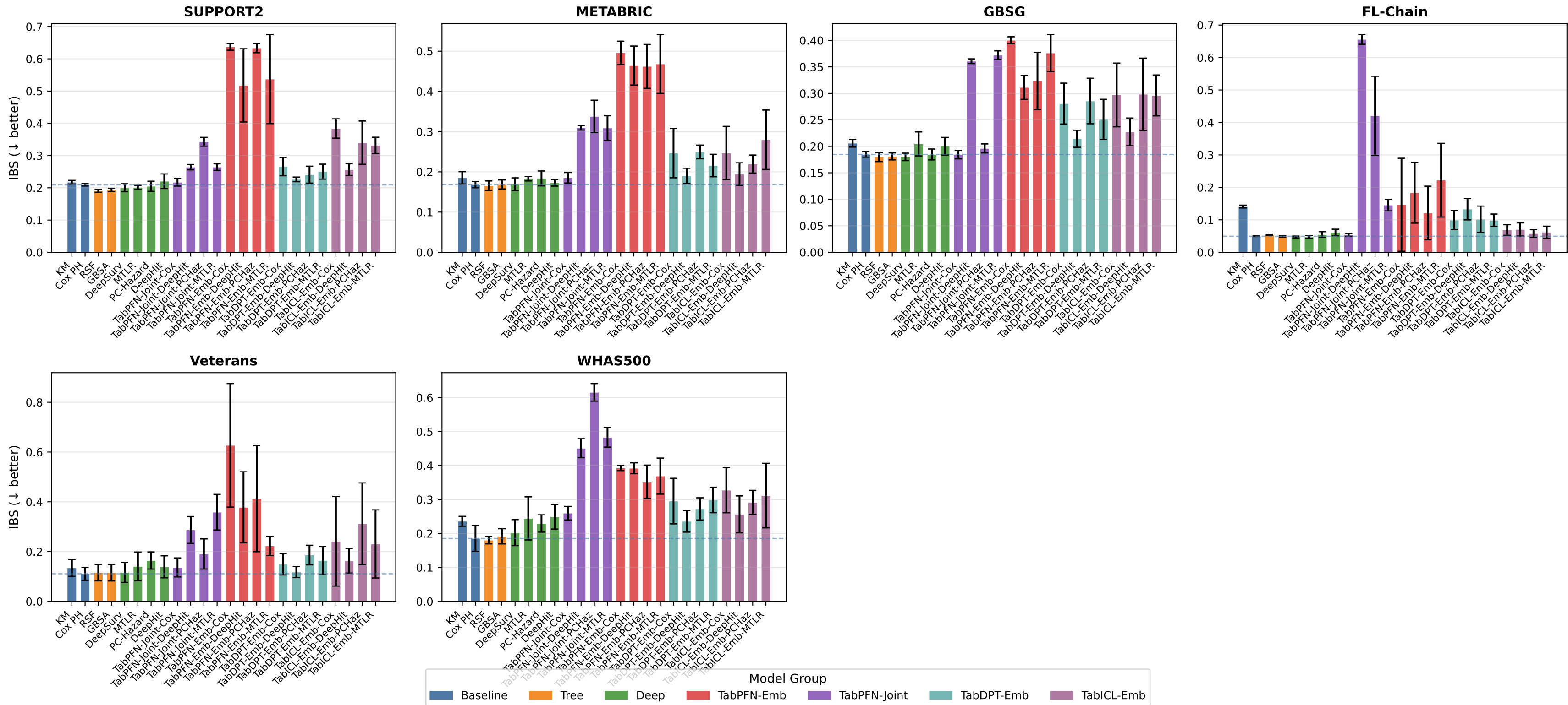
Integrated Brier Score — Lower is Better (mean \pm std, 5-fold CV)
