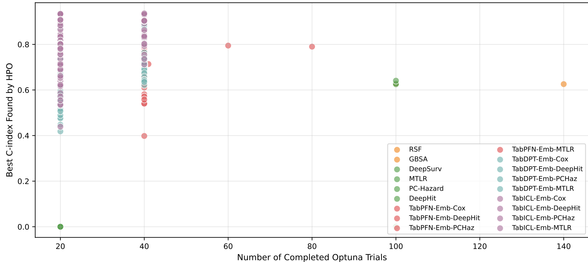
Convergence: Best C-index per Con (each point = model \times dataset \times fold)
