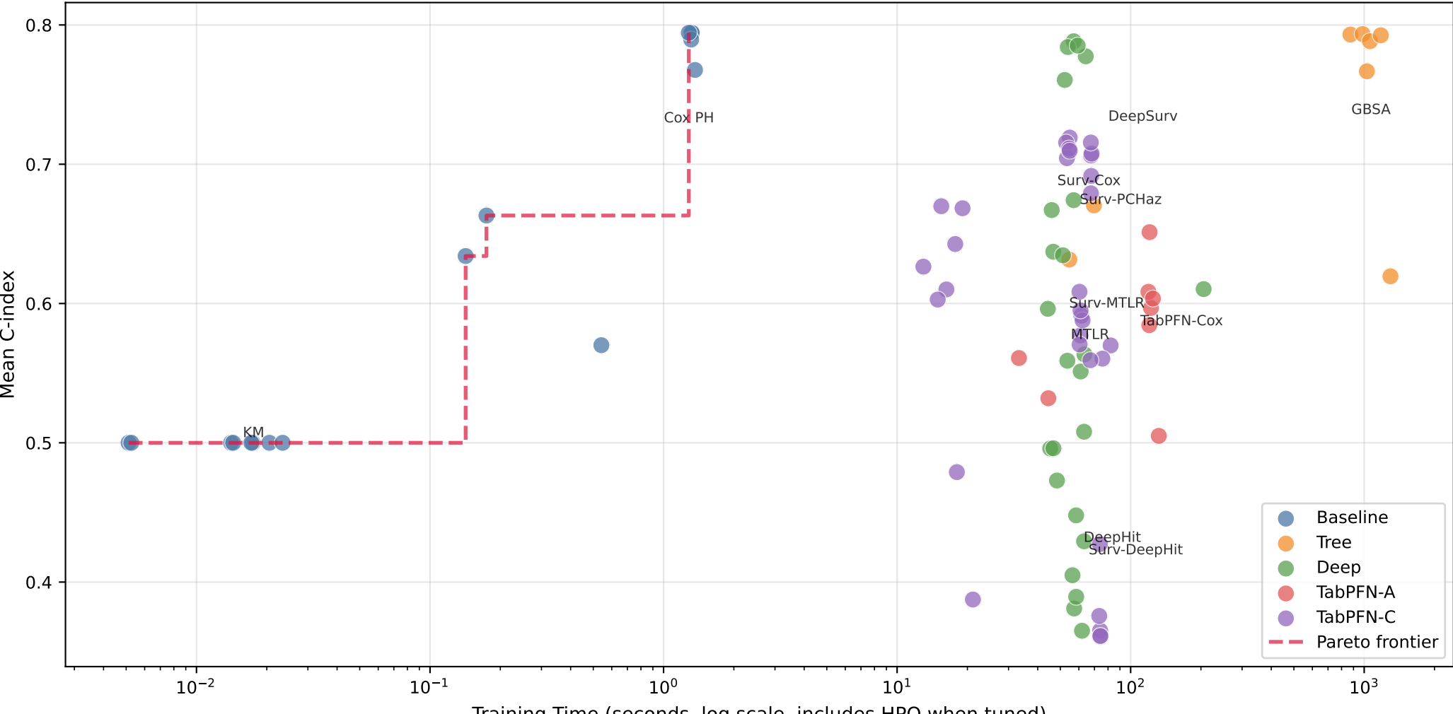
Performance-Efficiency Frontier (each point = model \times dataset mean)
