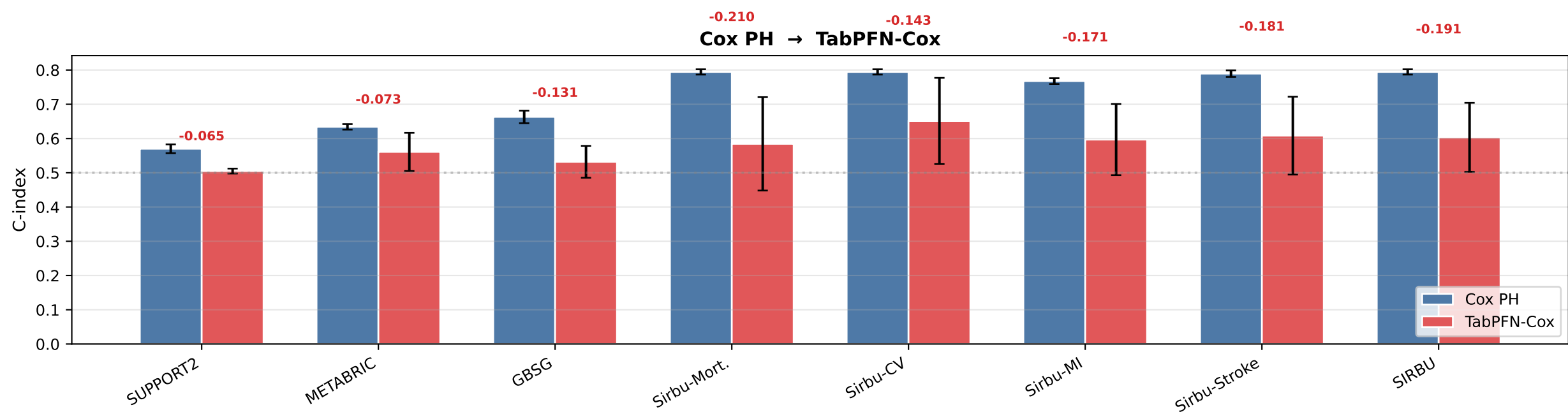
TabPFN Ablation: Classical vs Foundation Model Counterparts ( \Delta C-index shown above bars; green = improvement, red = degradation)
