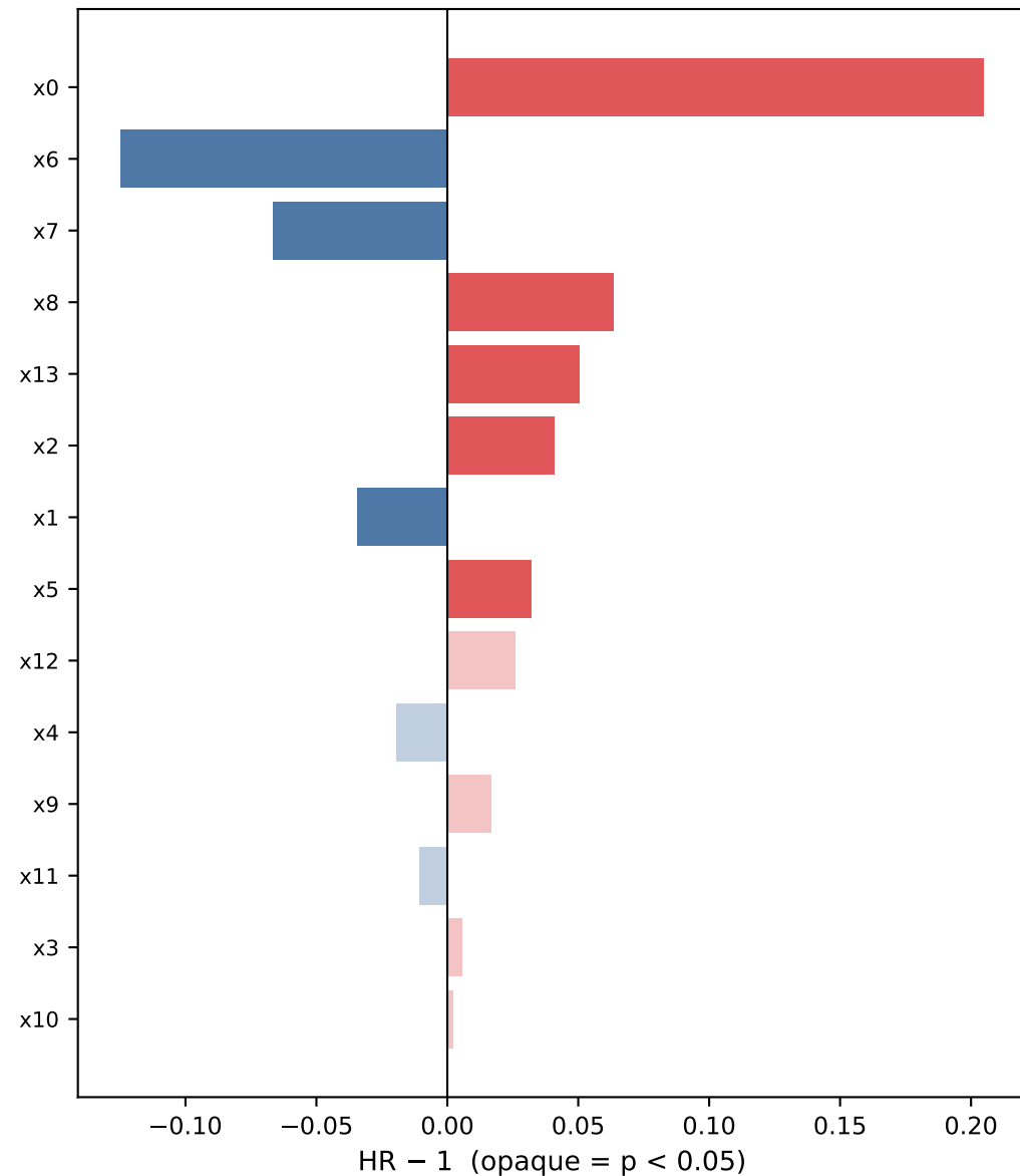
Cox PH Hazard Ratios
