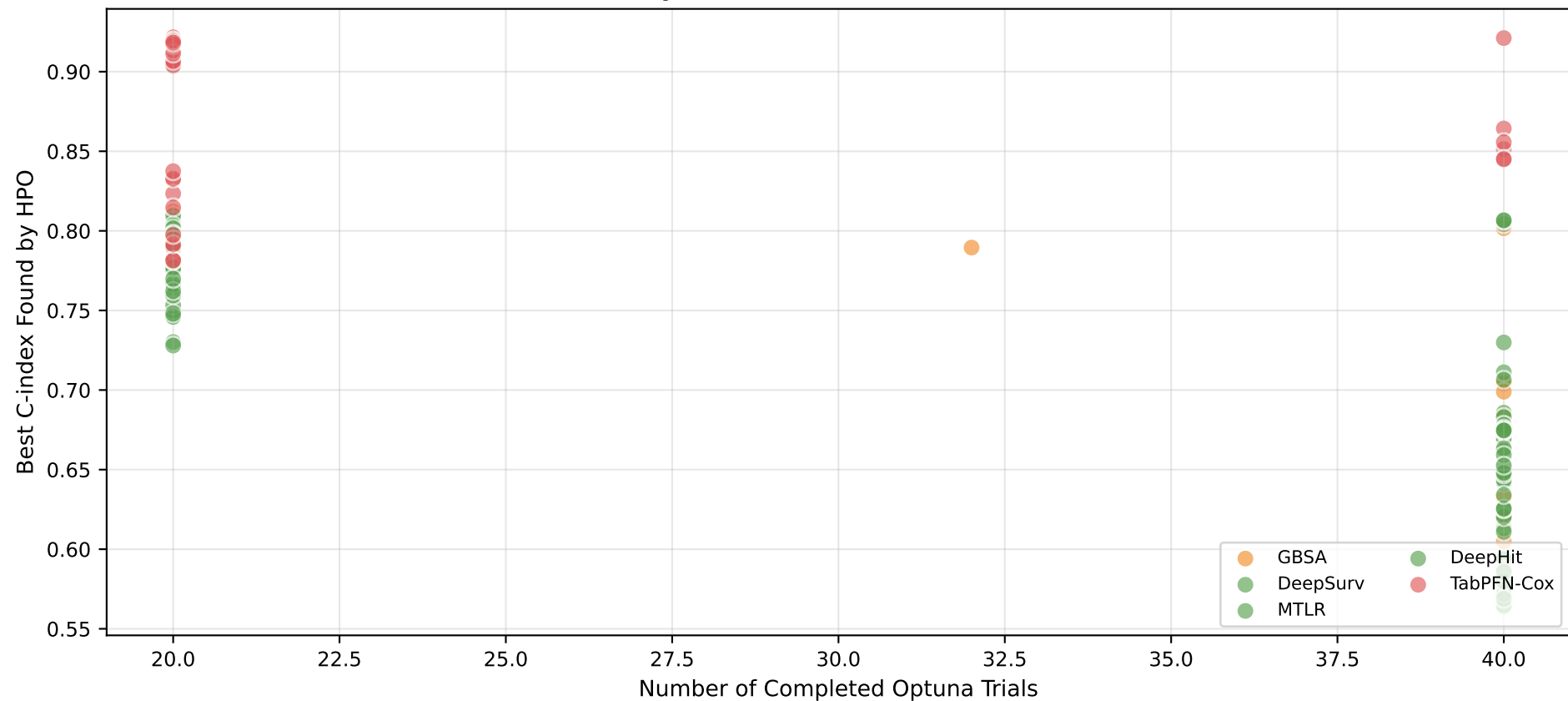
HPO Convergence: Best C-index per Completed Trials (each point = model \times dataset \times fold)
