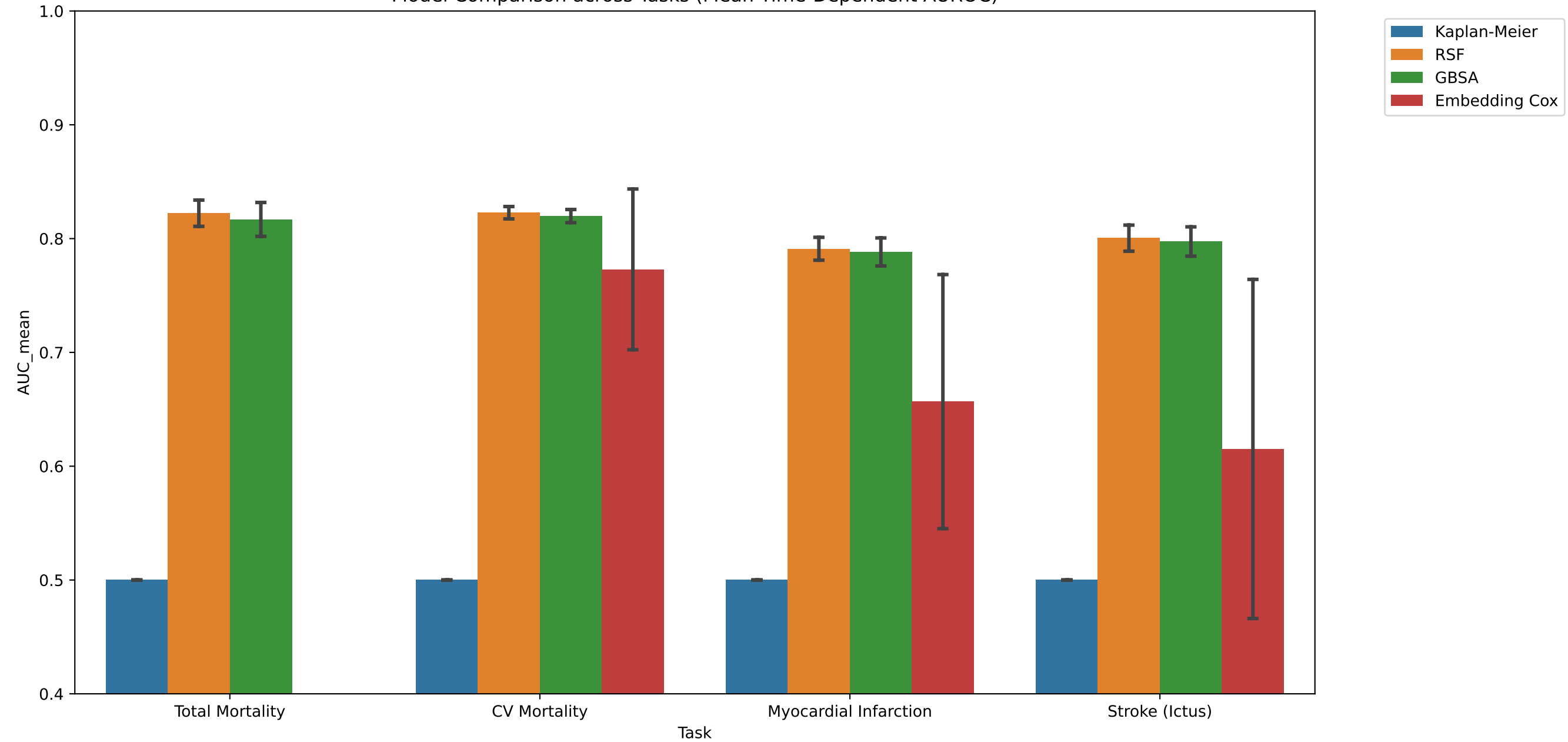
Model Comparison across Tasks (Mean Time-Dependent AUROC)
