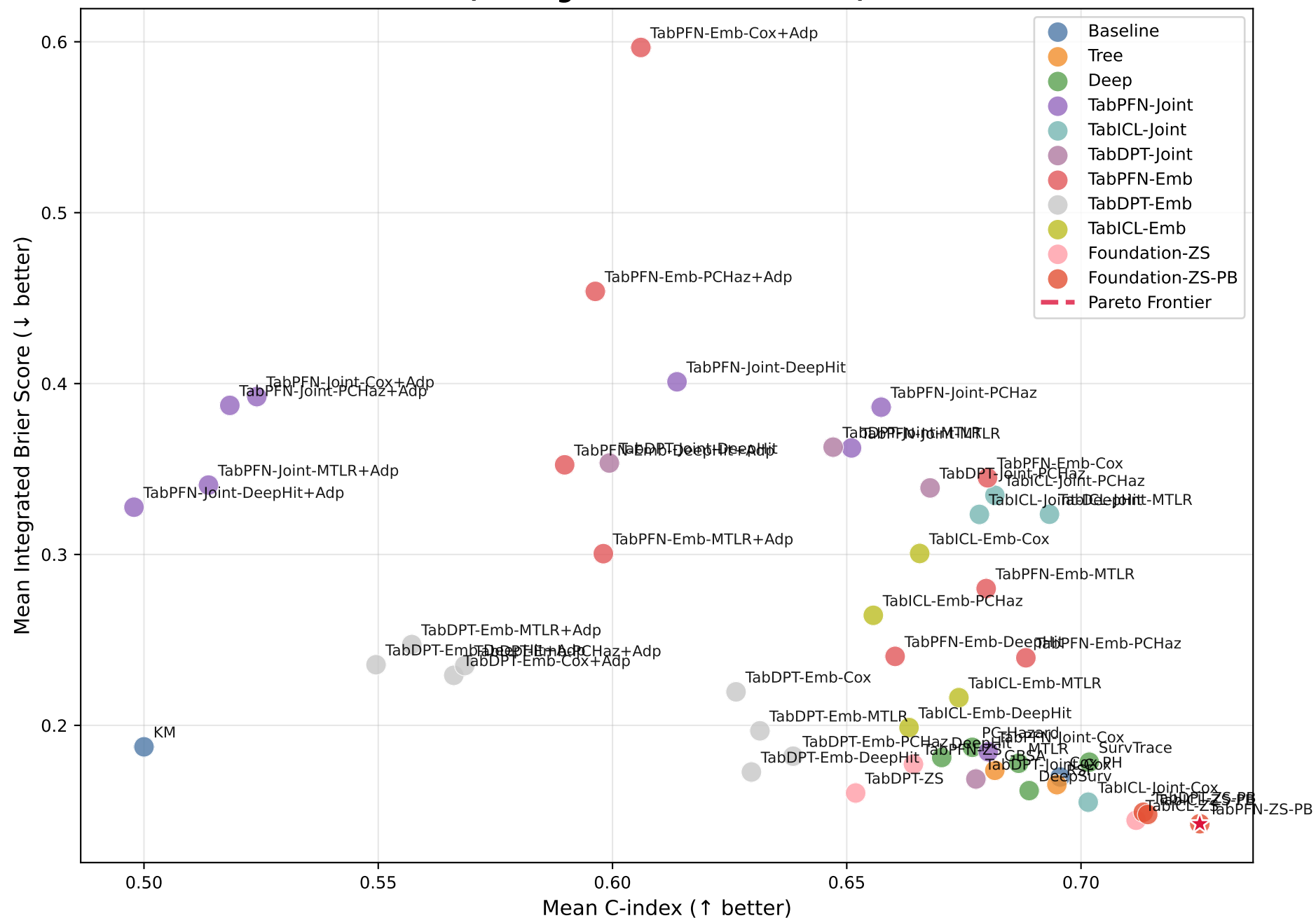
Pareto Frontier: Performance (C-index) vs Calibration (IBS) (Average across all datasets)
