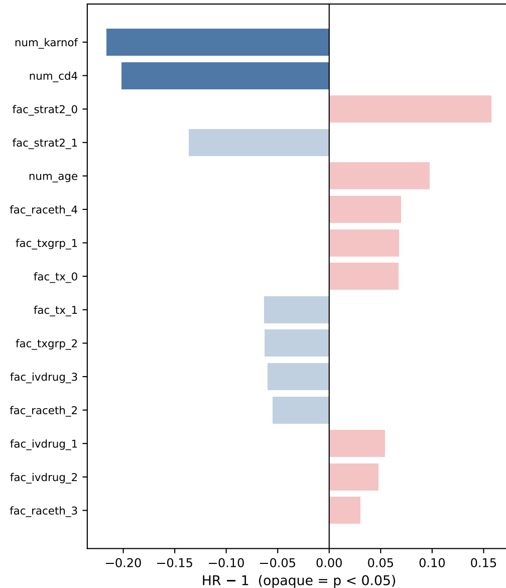
Cox PH Hazard Ratios
