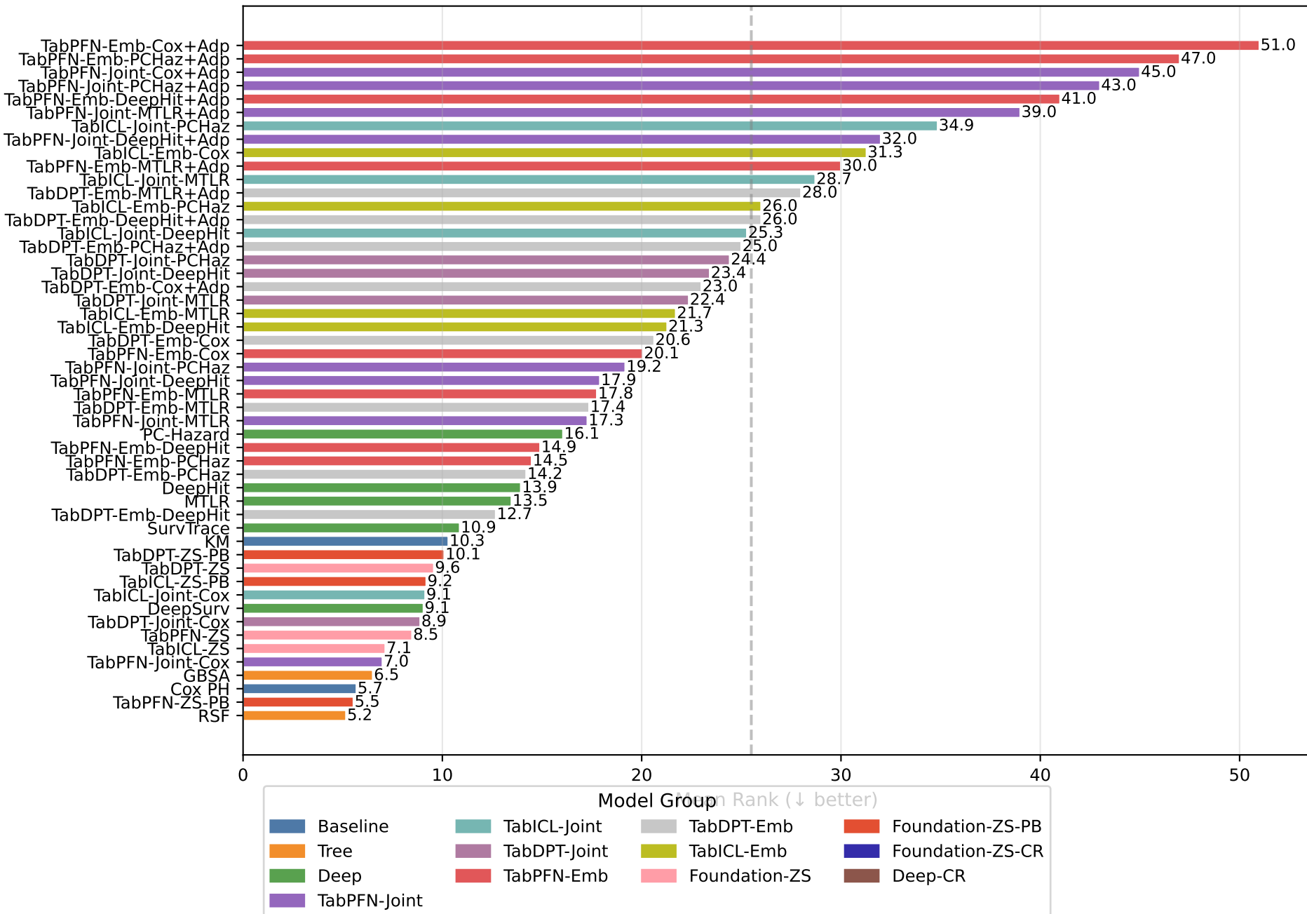
Average Model Rank Across All Datasets (ranked by IBS within each dataset, lowest=1)
