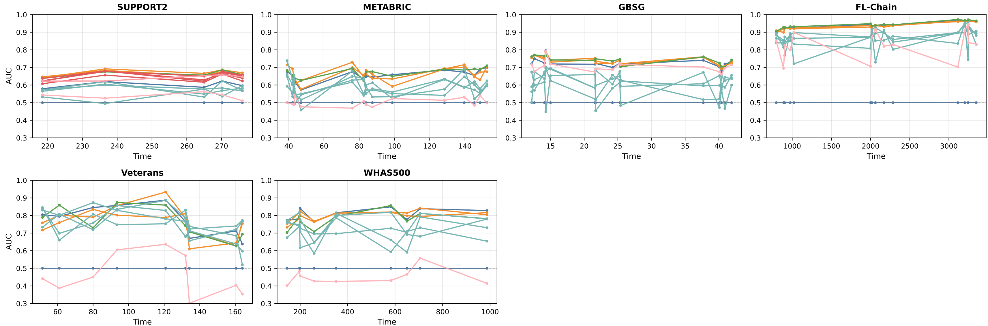
Time-dependent AUROC (mean across 5 folds)
