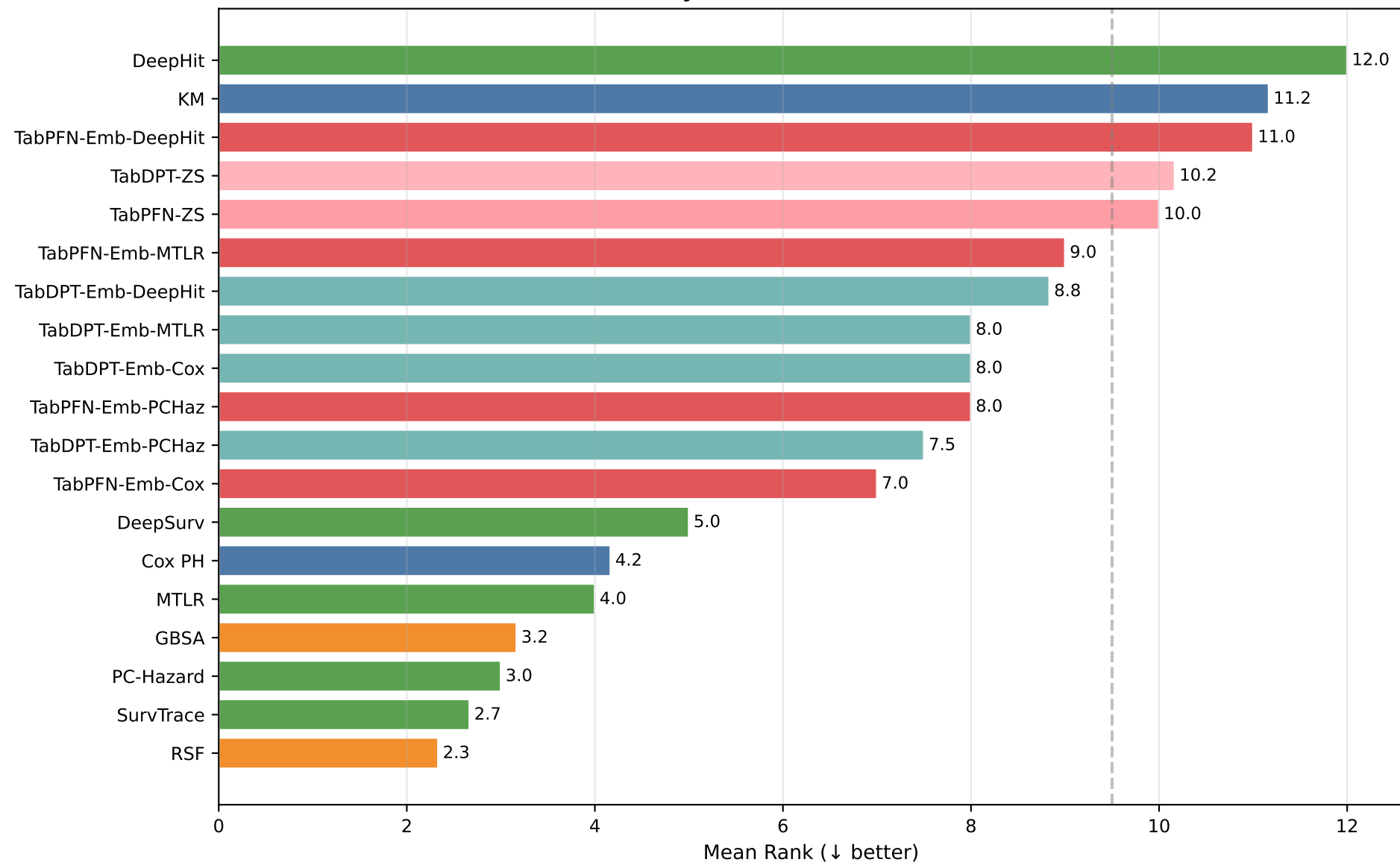
Average Model Rank Across All Datasets (ranked by C-index within each dataset)
