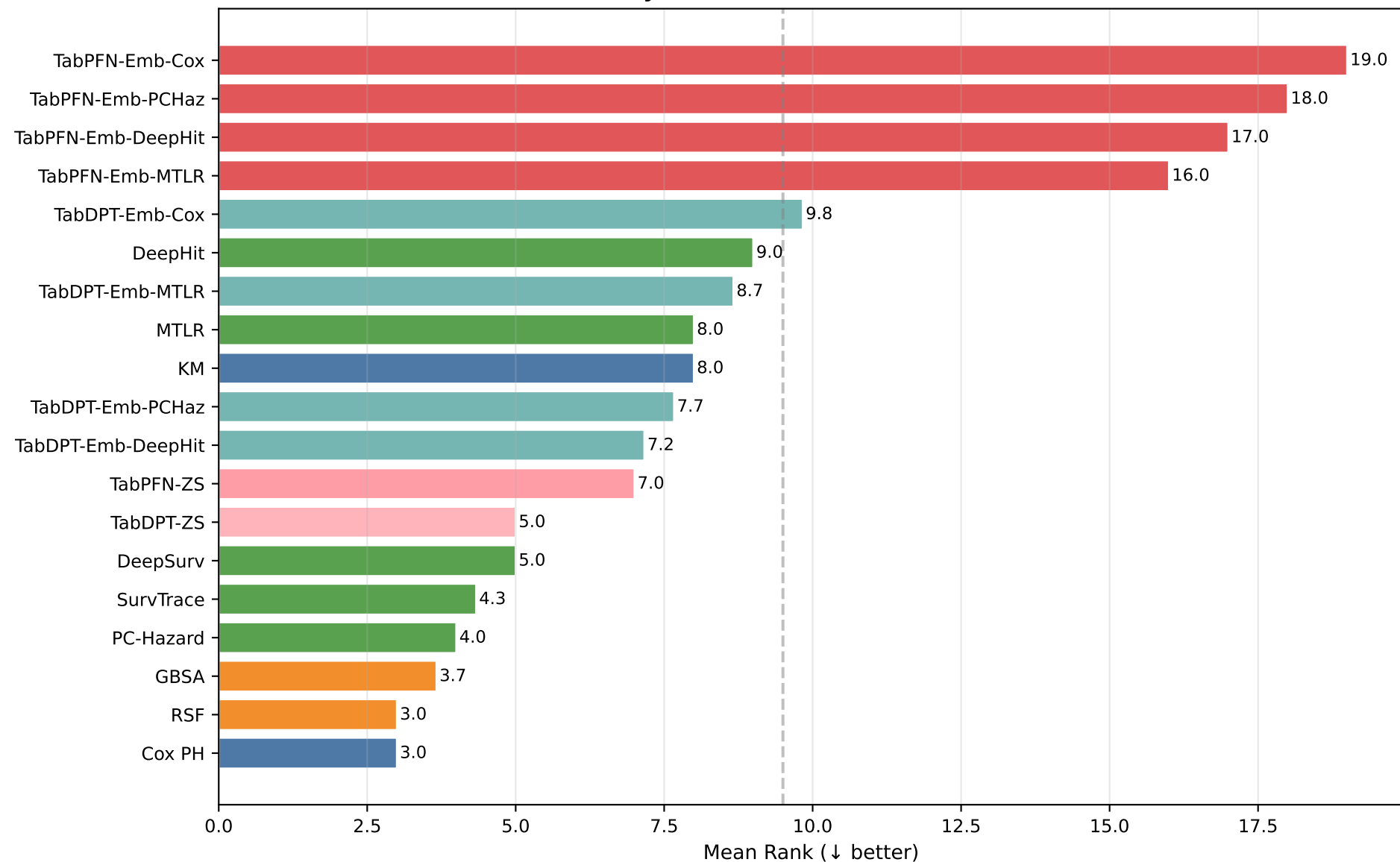
Average Model Rank Across All Datasets (ranked by IBS within each dataset, lowest=1)
