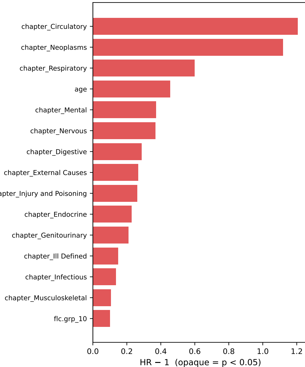
Cox PH Hazard Ratios
