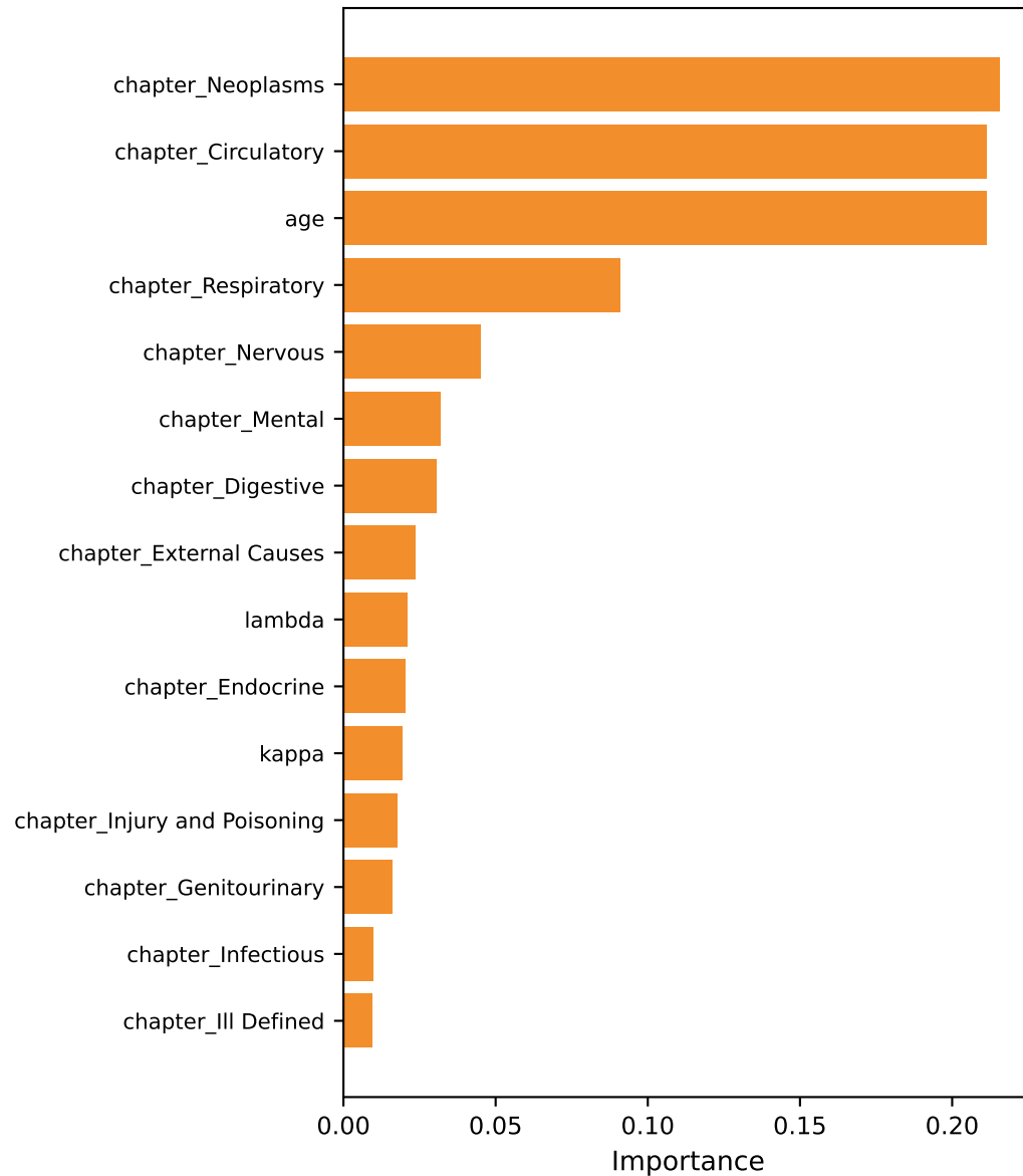
GBSA Feature Importance
