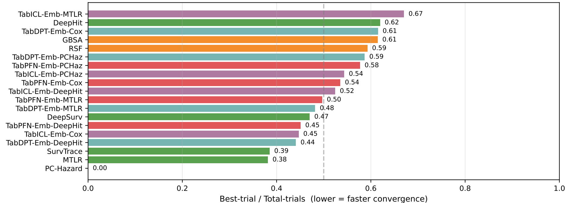
HPO Convergence Speed — Where Was the Best Trial Found?
