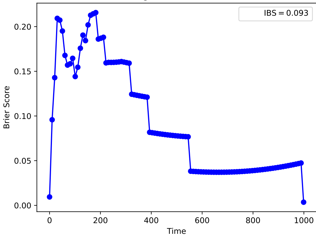
Integrated Brier Score
