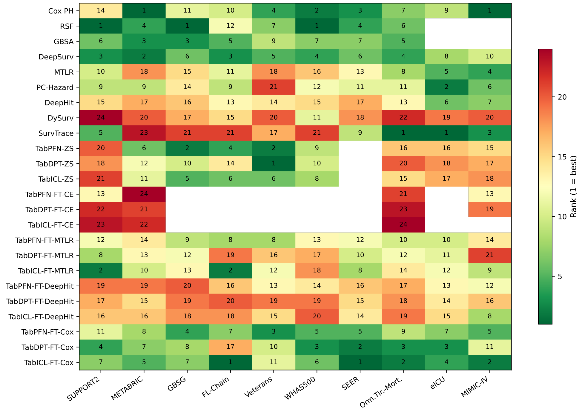
Model Rank per Dataset (IBS)
