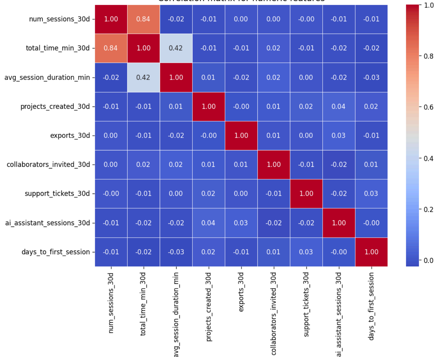
Correlation matrix for numeric features
