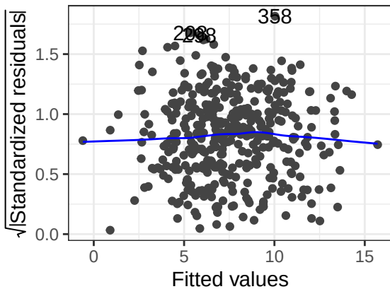
Scale-Location
