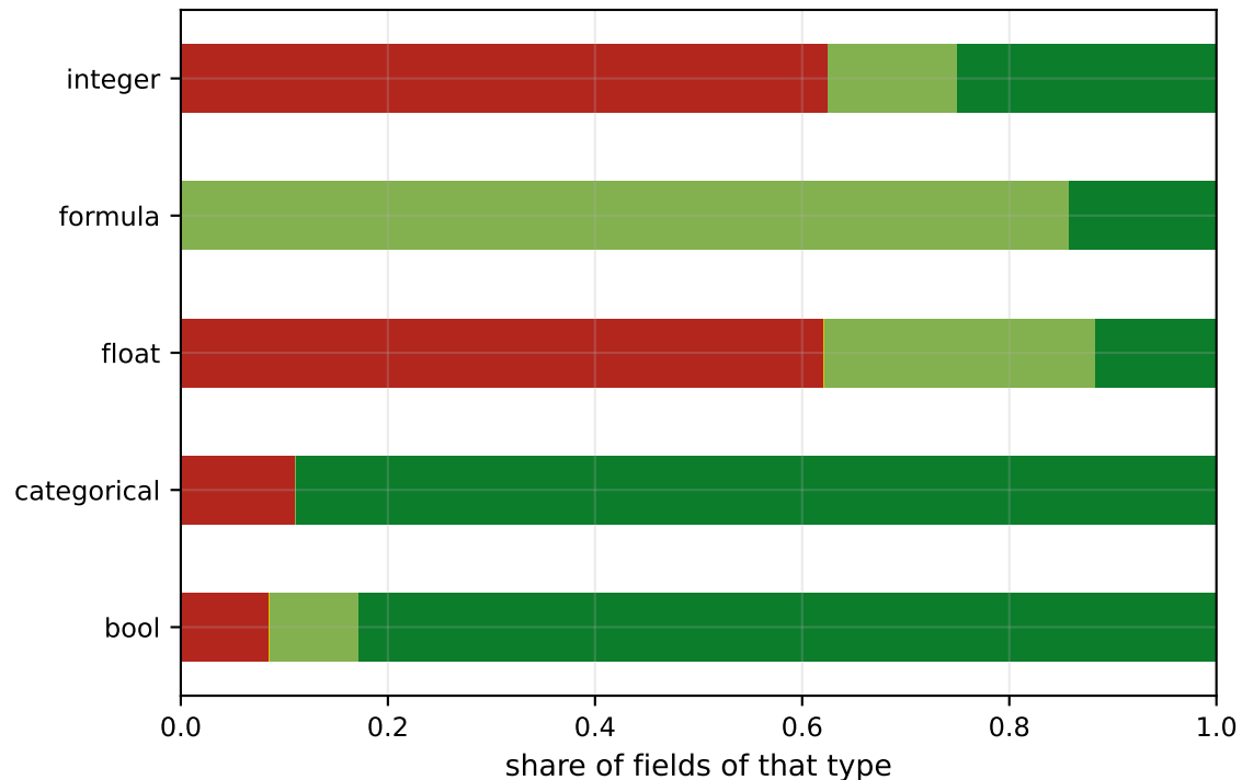
Difficulty composition by result type
