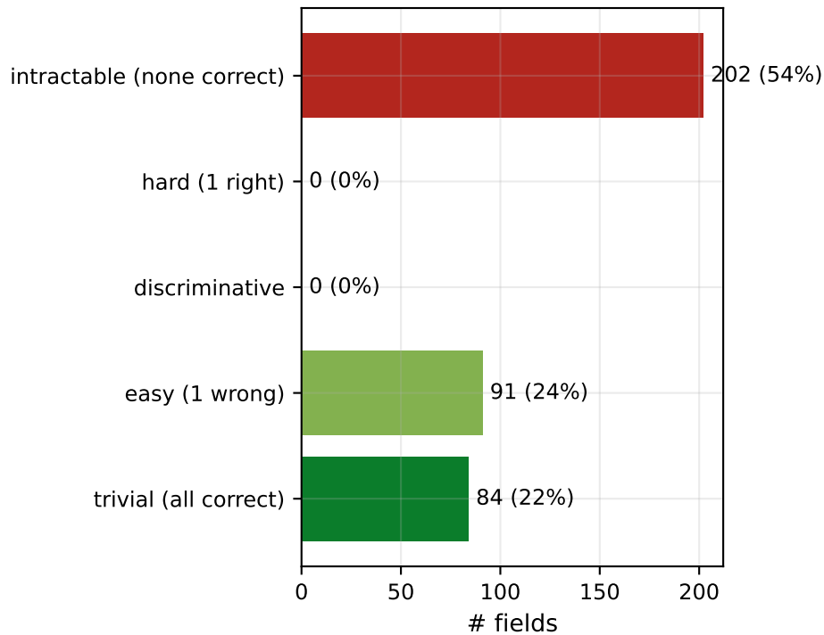
All 377 fields (per-field counts)
