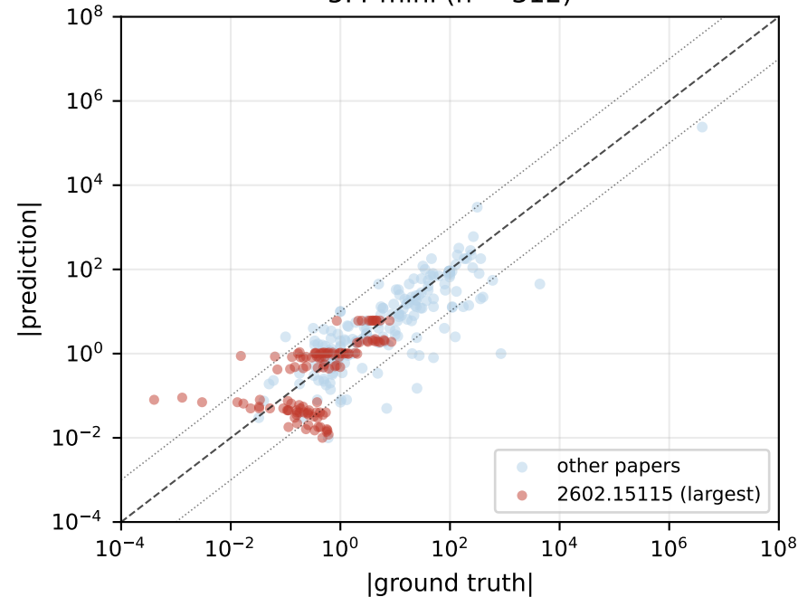
5.4-mini (n = 312)
