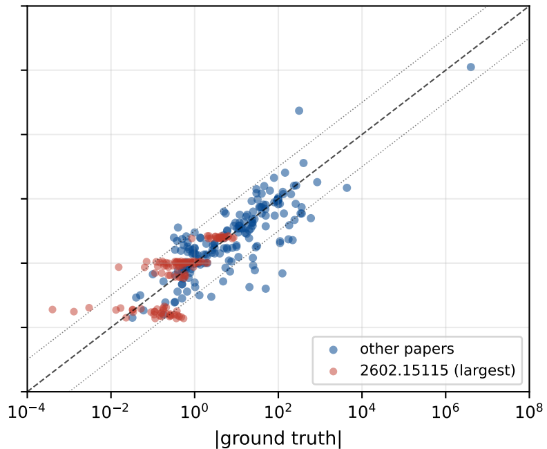
5.4-nano (n = 314)
