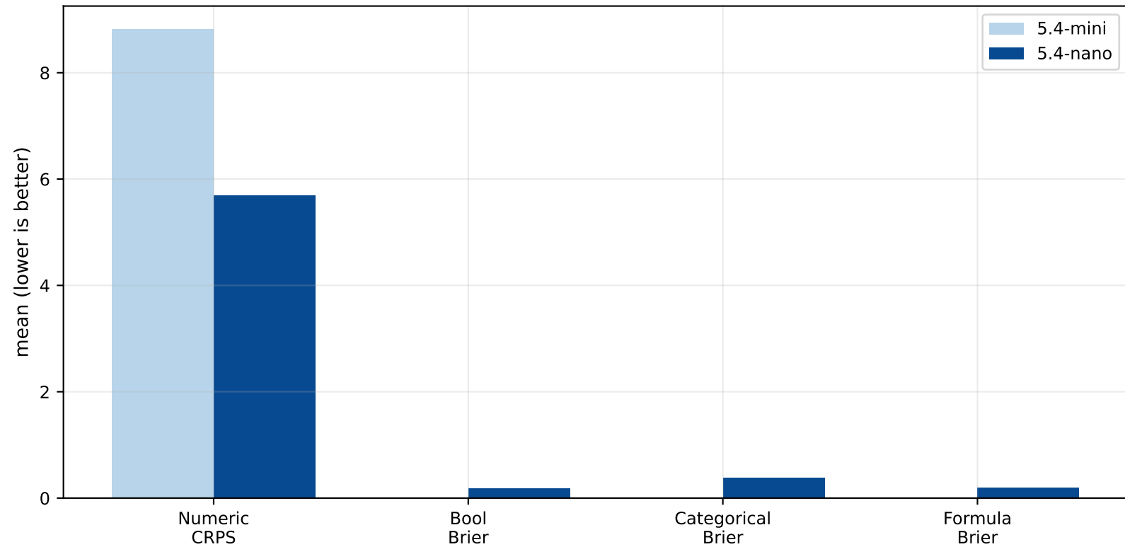
Per-model proper scoring rules — paper-macro of experiment-macro
