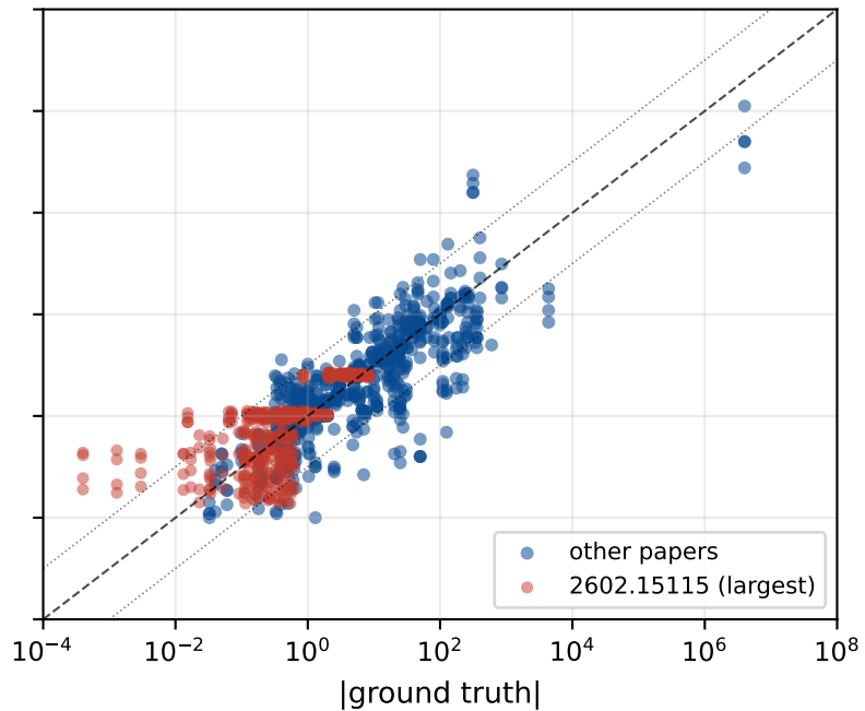
5.4-nano (n = 1230)
