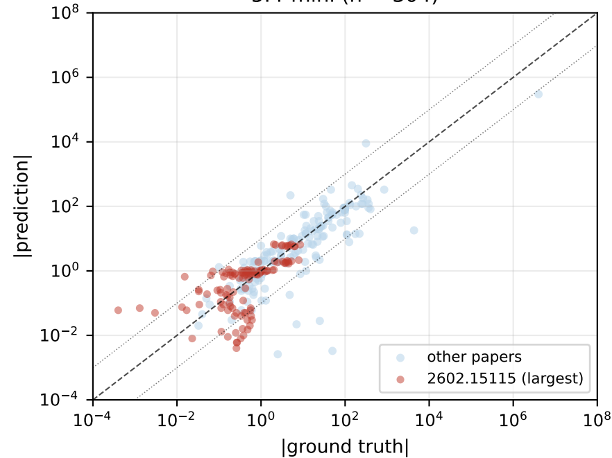
5.4-mini (n = 304)
