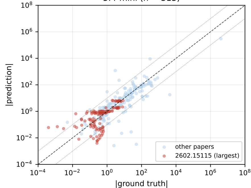
5.4-mini (n = 313)
