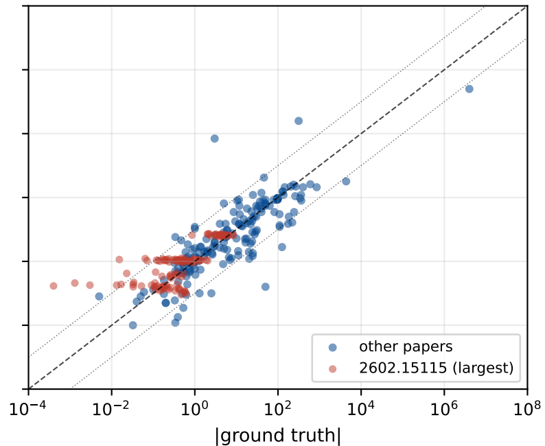
5.4-nano (n = 315)
