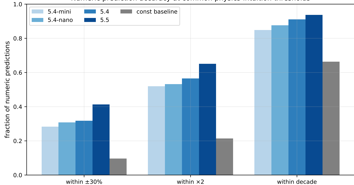
Numeric prediction accuracy at common physics-intuition thresholds
