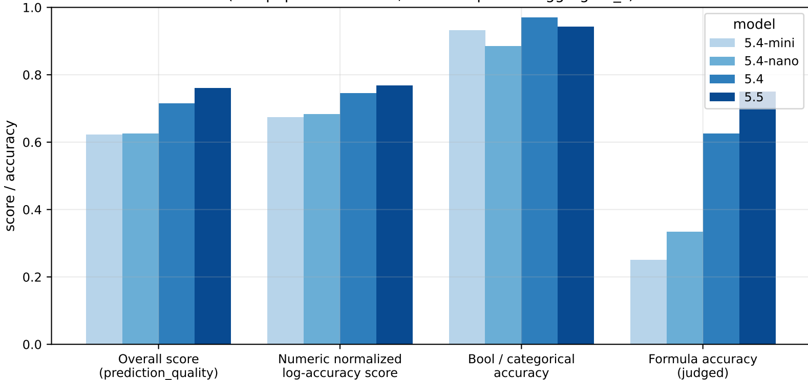
Aggregate benchmark performance by model — paper-macro (one paper = one vote; matches per-run aggregate_*)
