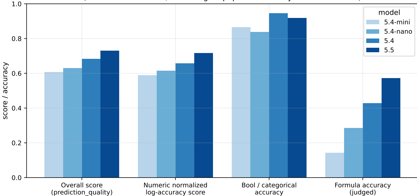
Aggregate benchmark performance by model — per-field micro (one field = one vote; over-weights papers with many redundant fields)
