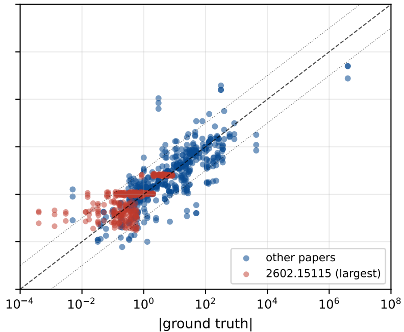
5.4-nano (n = 943)
