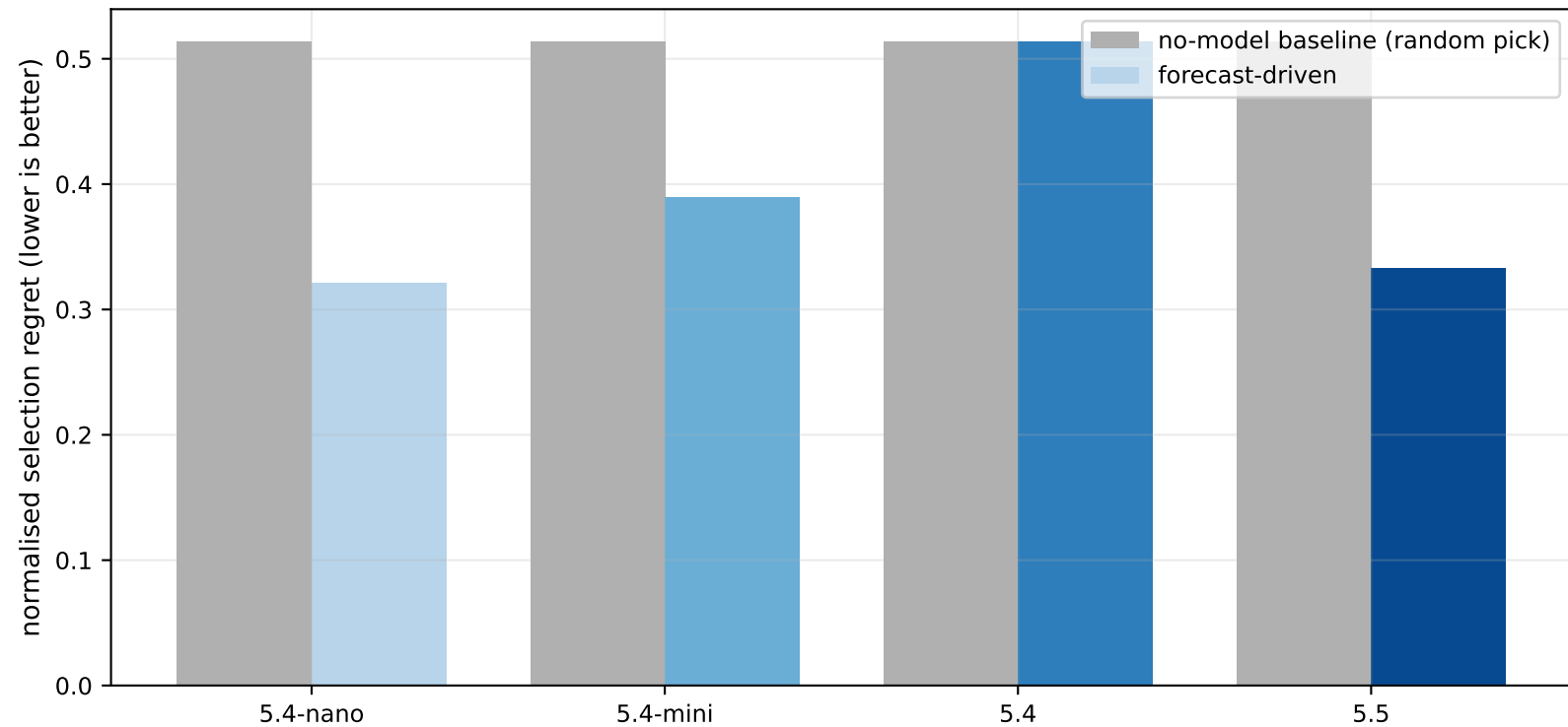
Experiment-selection regret: forecast-driven vs. no-model baseline (gap = decision value added by the forecaster)
