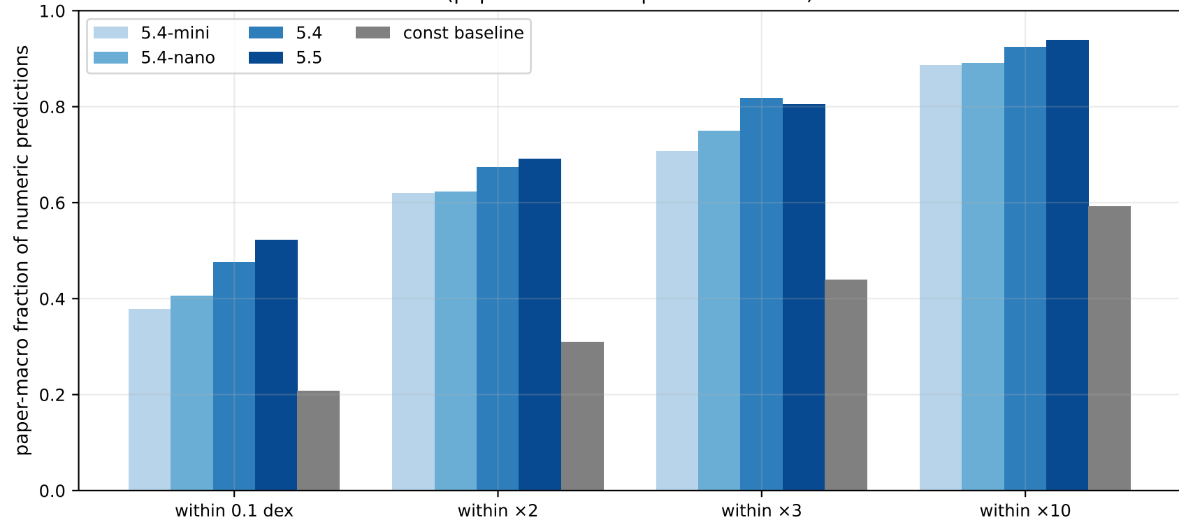
Numeric prediction accuracy at common physics-intuition thresholds (paper-macro of experiment-macro)
