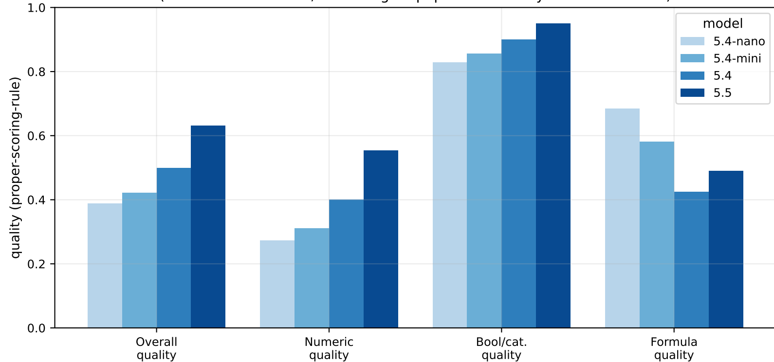
Aggregate quality by model — per-field micro (one field = one vote; over-weights papers with many redundant fields)
