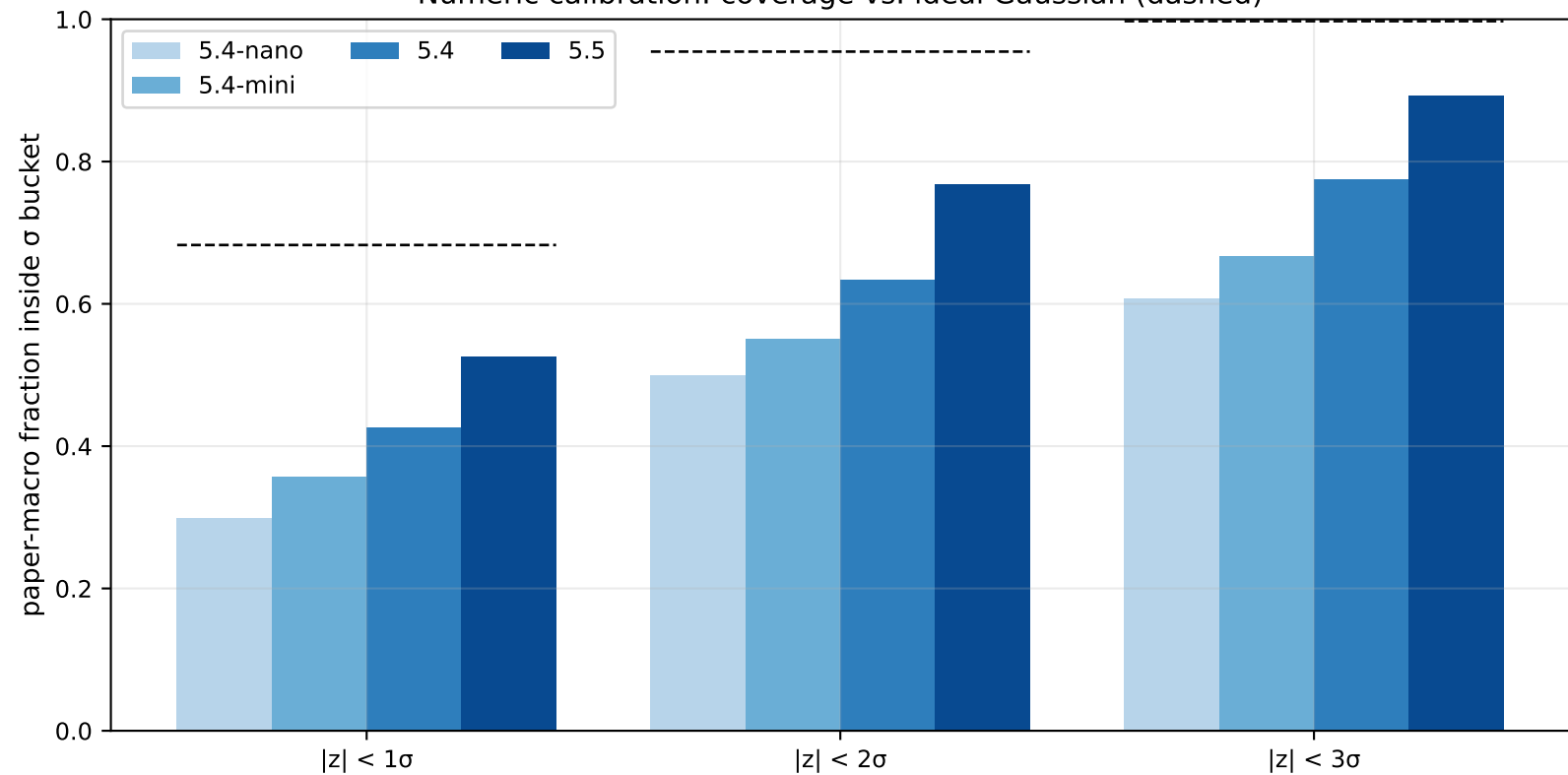
Numeric calibration: coverage vs. ideal Gaussian (dashed)
