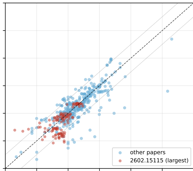
5.4-mini (n = 513)
