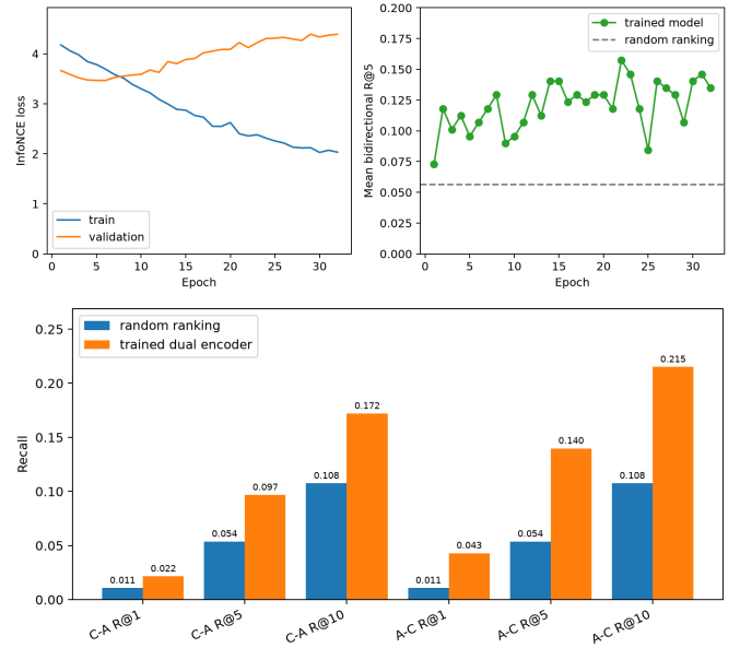
Fig. 7. Task 4 optimization (top) and held-out bidirectional retrieval compared with random ranking (bottom).
