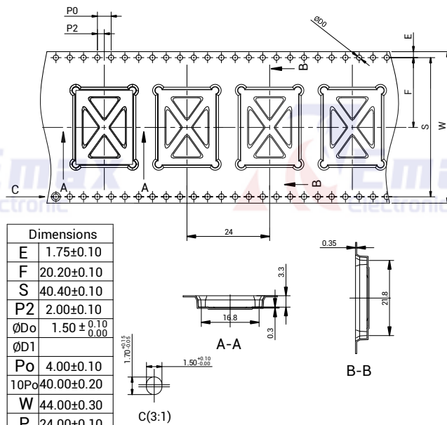
Figure 5-2 UM982 Package
