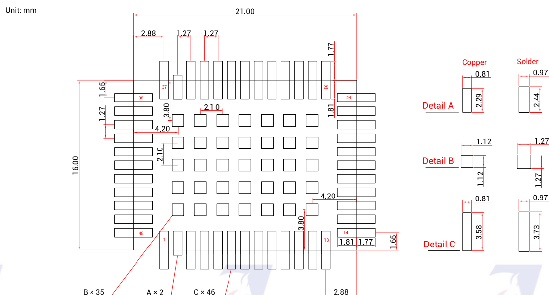
Figure 3-4 Recommended PCB Package Design
