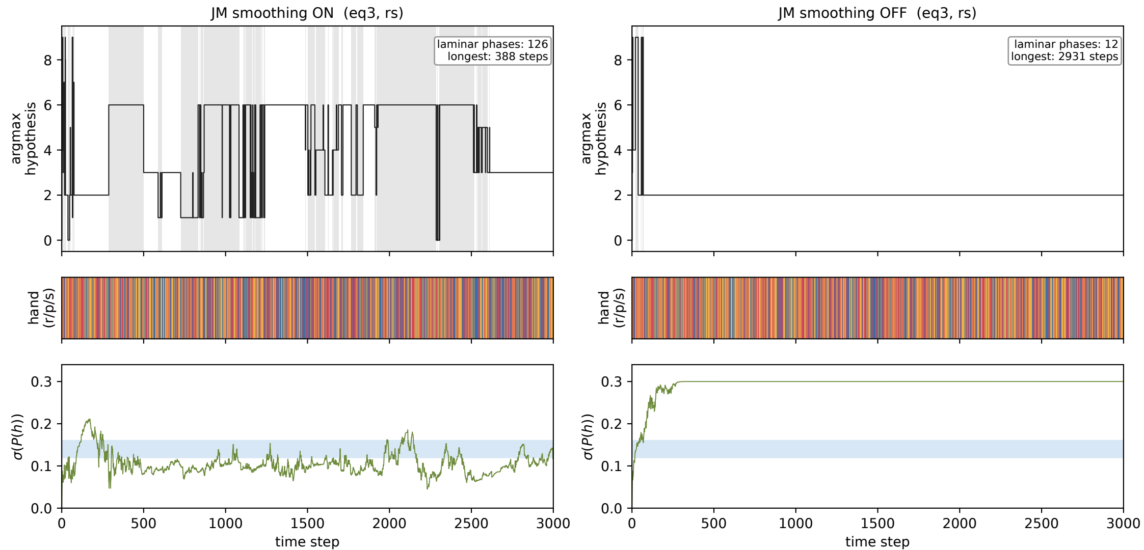
Hands / argmax / laminar structure under JM-on vs JM-off (bib--bib, rs, tie=skip, N_h=10 , T=3000 , seed=1)
